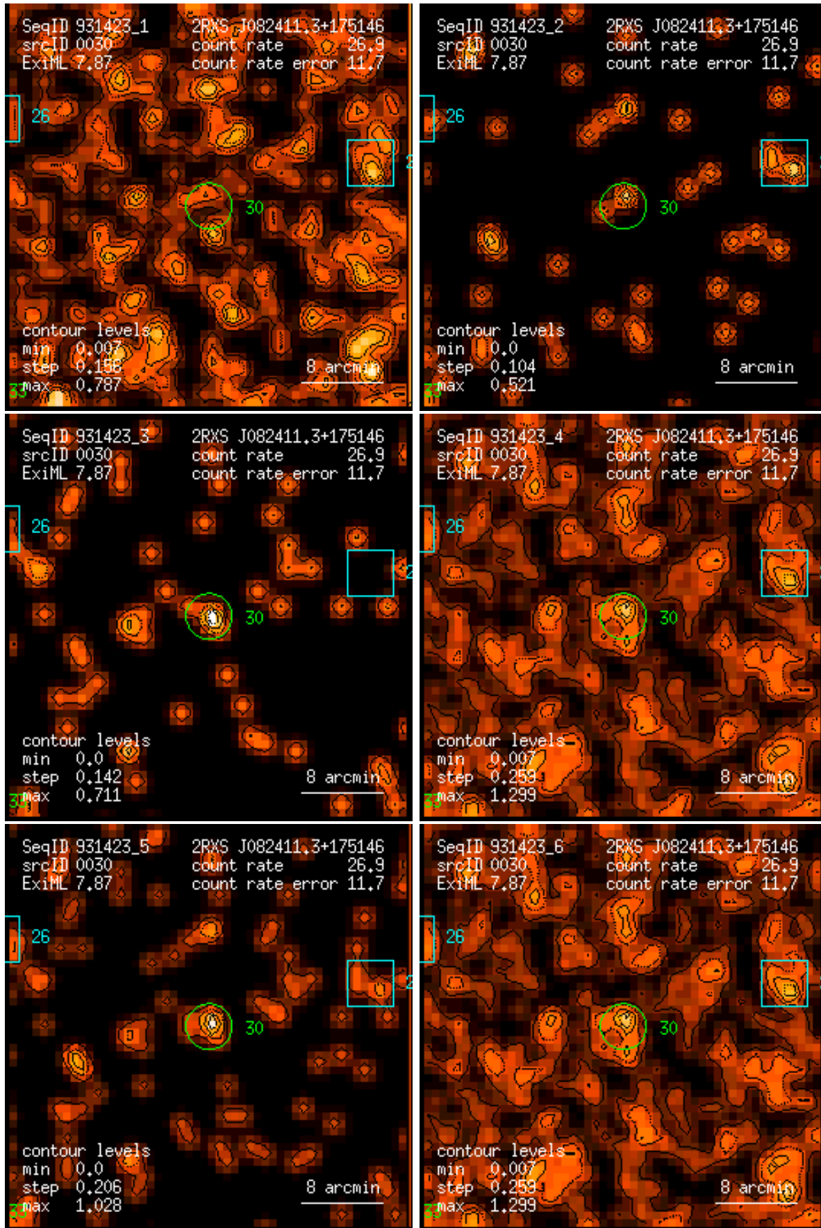
Figure 30: RASS 931423: detection 0030: band rate images, Gaussian filter: (1) PSPC channels 11 – 41, (2) 52 – 90, (3) 91 – 201, (4) 11 – 235, (5) 52 – 201, (6) 11 – 201. Broad band rates in counts/ks. Band rate contour levels in counts/ks/arcmin 2 .
