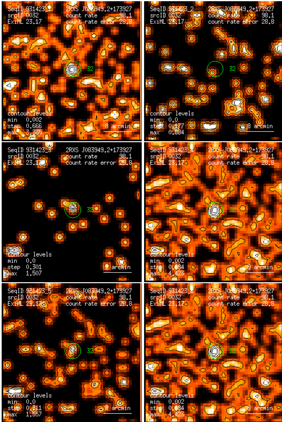
Figure 32: RASS 931423: detection 0032: band rate images, Gaussian filter: (1) PSPC channels 11 – 41, (2) 52 – 90, (3) 91 – 201, (4) 11 – 235, (5) 52 – 201, (6) 11 – 201. Broad band rates in counts/ks. Band rate contour levels in counts/ks/arcmin 2 .
