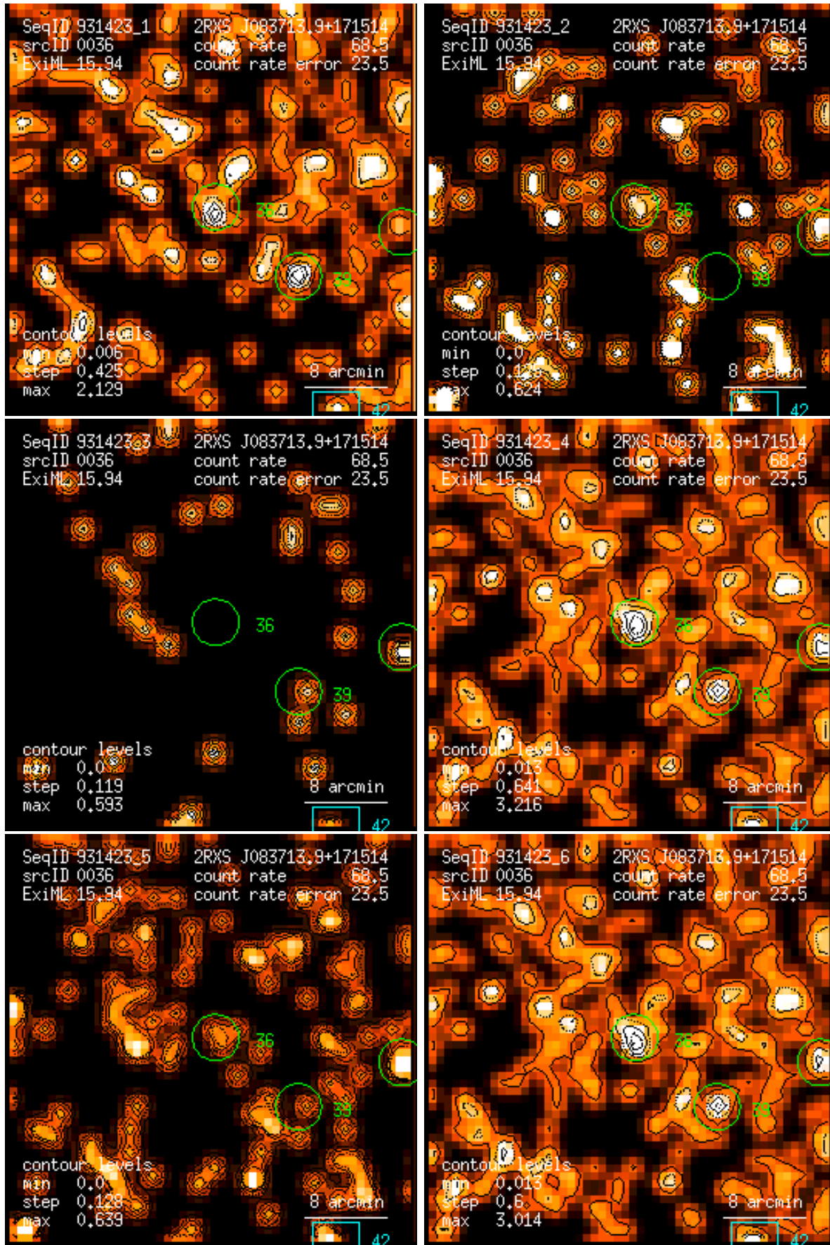
Figure 36: RASS 931423: detection 0036: band rate images, Gaussian filter: (1) PSPC channels 11 – 41, (2) 52 – 90, (3) 91 – 201, (4) 11 – 235, (5) 52 – 201, (6) 11 – 201. Broad band rates in counts/ks. Band rate contour levels in counts/ks/arcmin 2 .
