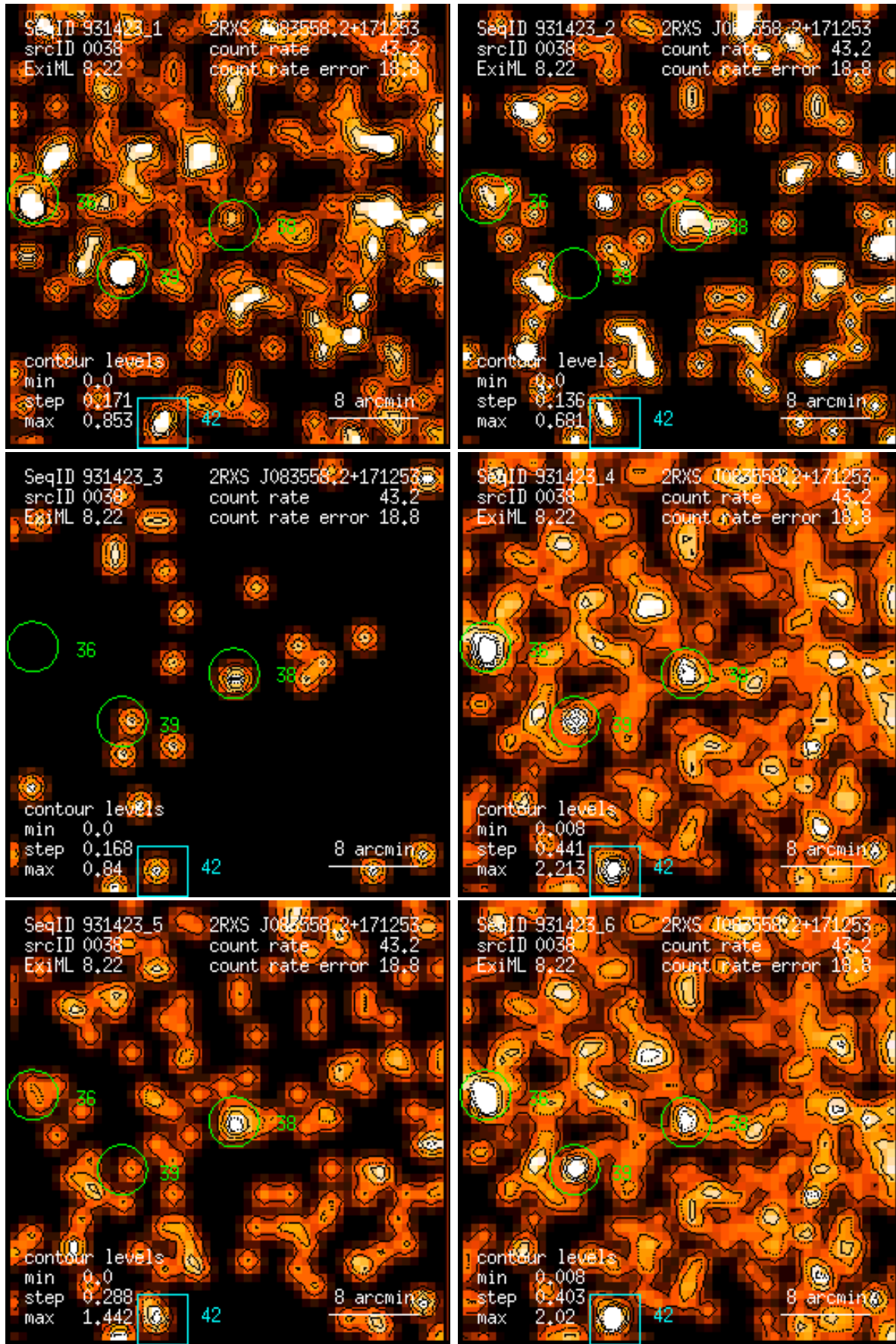
Figure 38: RASS 931423: detection 0038: band rate images, Gaussian filter: (1) PSPC channels 11 – 41, (2) 52 – 90, (3) 91 – 201, (4) 11 – 235, (5) 52 – 201, (6) 11 – 201. Broad band rates in counts/ks. Band rate contour levels in counts/ks/arcmin 2 .
