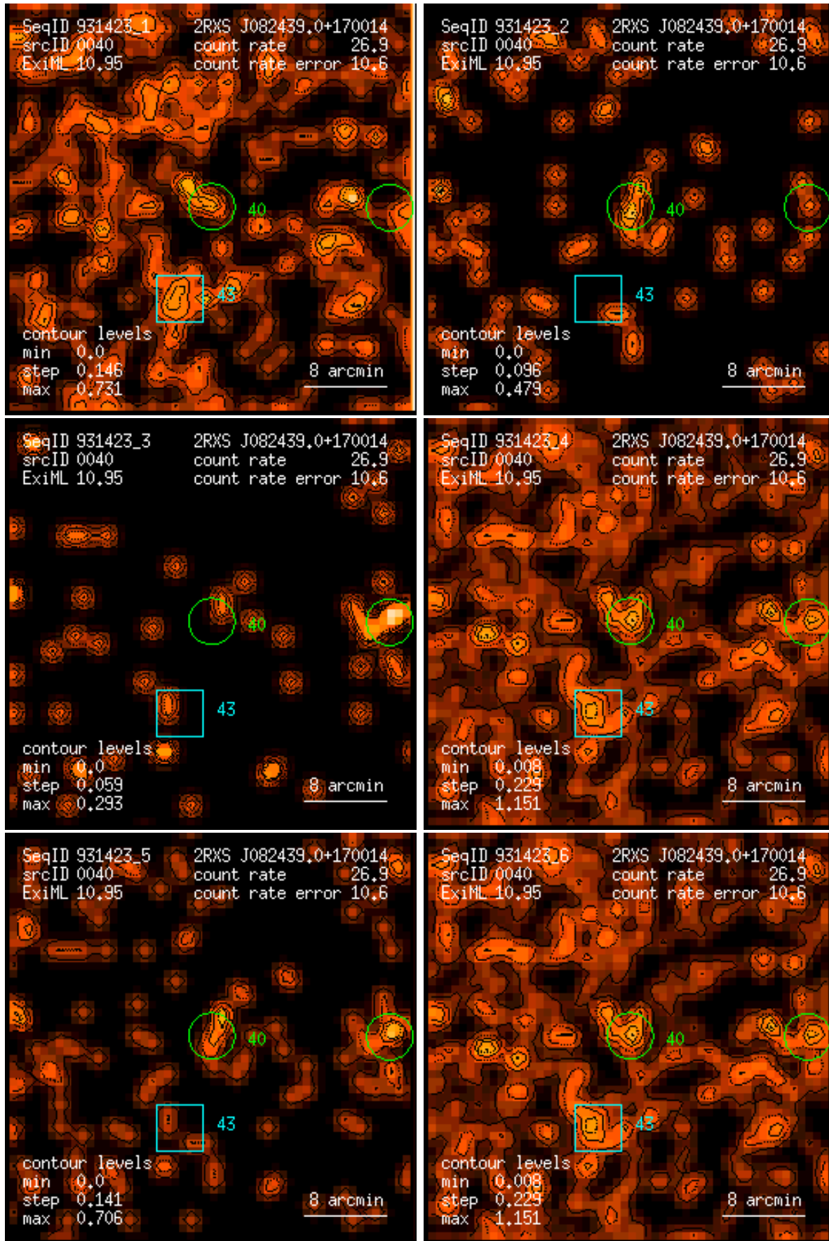
Figure 40: RASS 931423: detection 0040: band rate images, Gaussian filter: (1) PSPC channels 11 – 41, (2) 52 – 90, (3) 91 – 201, (4) 11 – 235, (5) 52 – 201, (6) 11 – 201. Broad band rates in counts/ks. Band rate contour levels in counts/ks/arcmin 2 .
