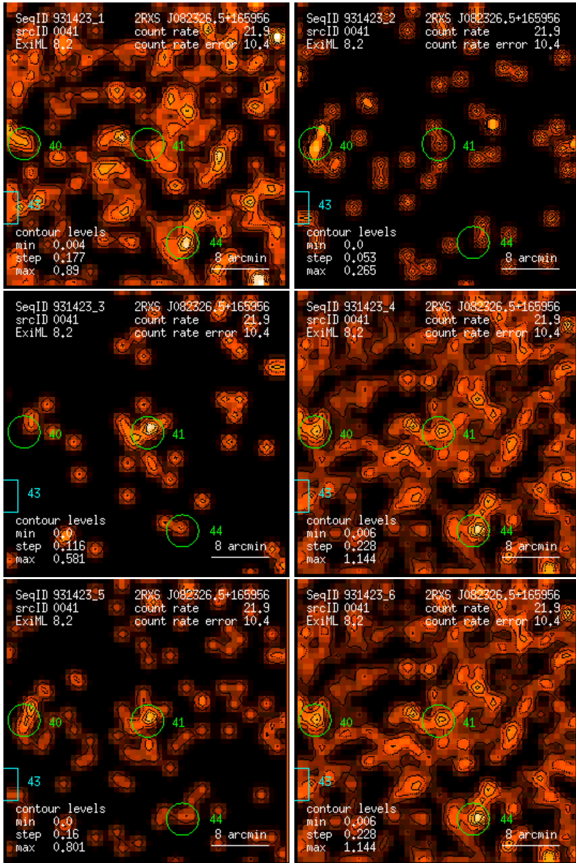
Figure 41: RASS 931423: detection 0041: band rate images, Gaussian filter: (1) PSPC channels 11 – 41, (2) 52 – 90, (3) 91 – 201, (4) 11 – 235, (5) 52 – 201, (6) 11 – 201. Broad band rates in counts/ks. Band rate contour levels in counts/ks/arcmin 2 .
