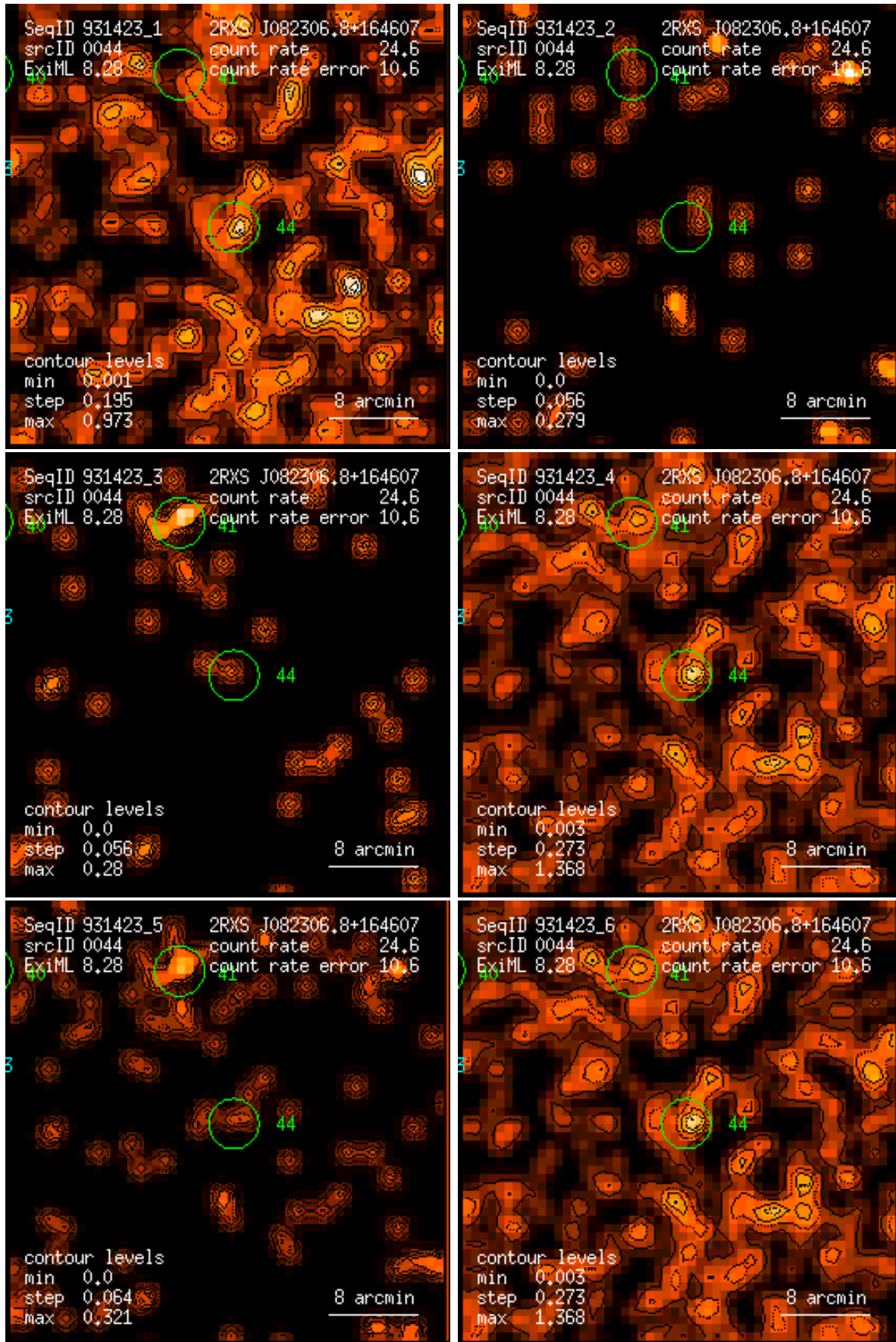
Figure 44: RASS 931423: detection 0044: band rate images, Gaussian filter: (1) PSPC channels 11 – 41, (2) 52 – 90, (3) 91 – 201, (4) 11 – 235, (5) 52 – 201, (6) 11 – 201. Broad band rates in counts/ks. Band rate contour levels in counts/ks/arcmin 2 .
