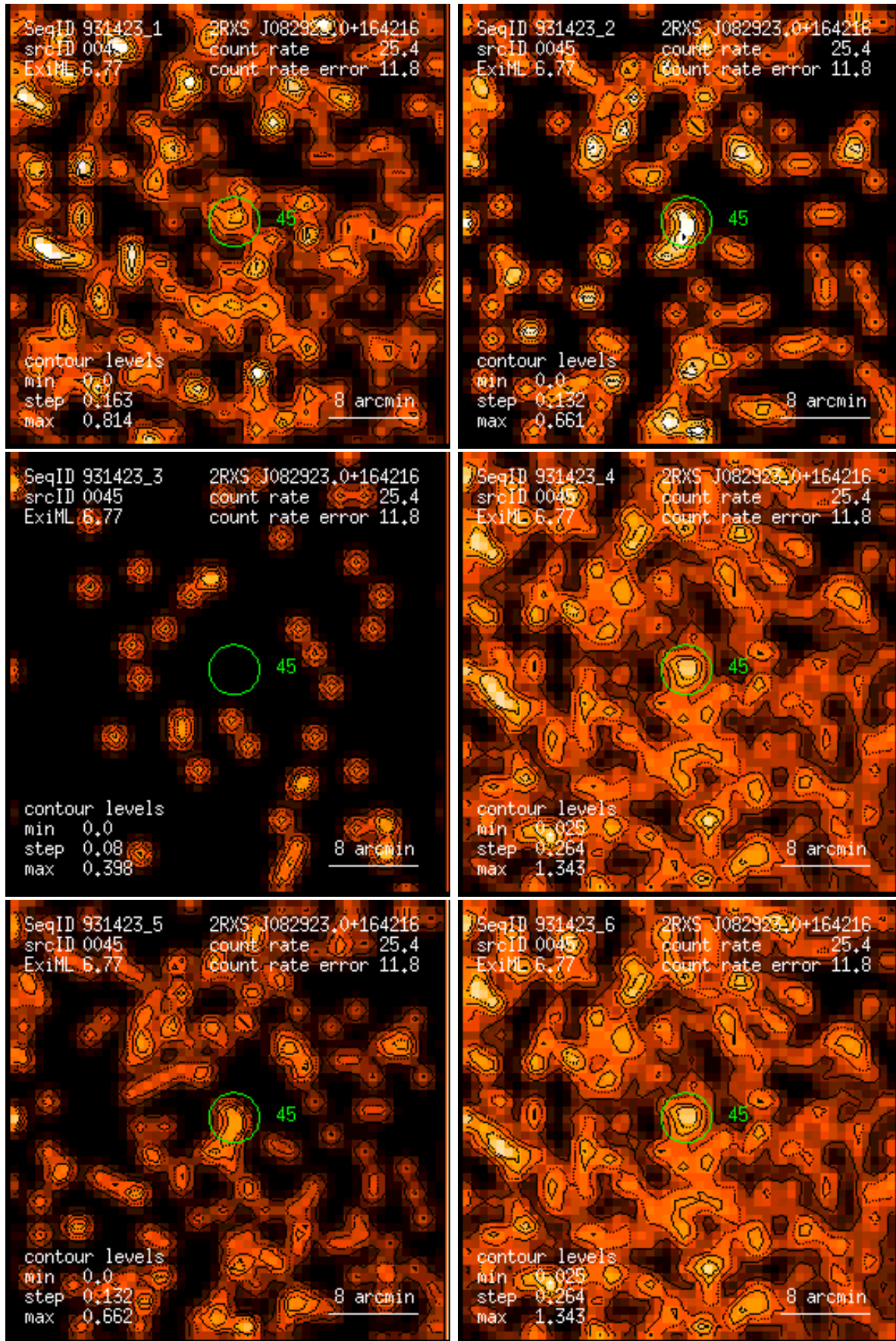
Figure 45: RASS 931423: detection 0045: band rate images, Gaussian filter: (1) PSPC channels 11 – 41, (2) 52 – 90, (3) 91 – 201, (4) 11 – 235, (5) 52 – 201, (6) 11 – 201. Broad band rates in counts/ks. Band rate contour levels in counts/ks/arcmin 2 .
