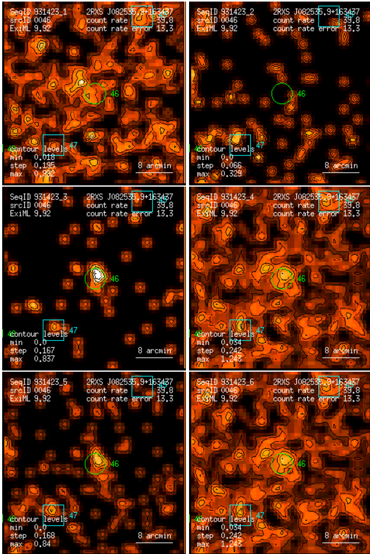
Figure 46: RASS 931423: detection 0046: band rate images, Gaussian filter: (1) PSPC channels 11 – 41, (2) 52 – 90, (3) 91 – 201, (4) 11 – 235, (5) 52 – 201, (6) 11 – 201. Broad band rates in counts/ks. Band rate contour levels in counts/ks/arcmin 2 .
