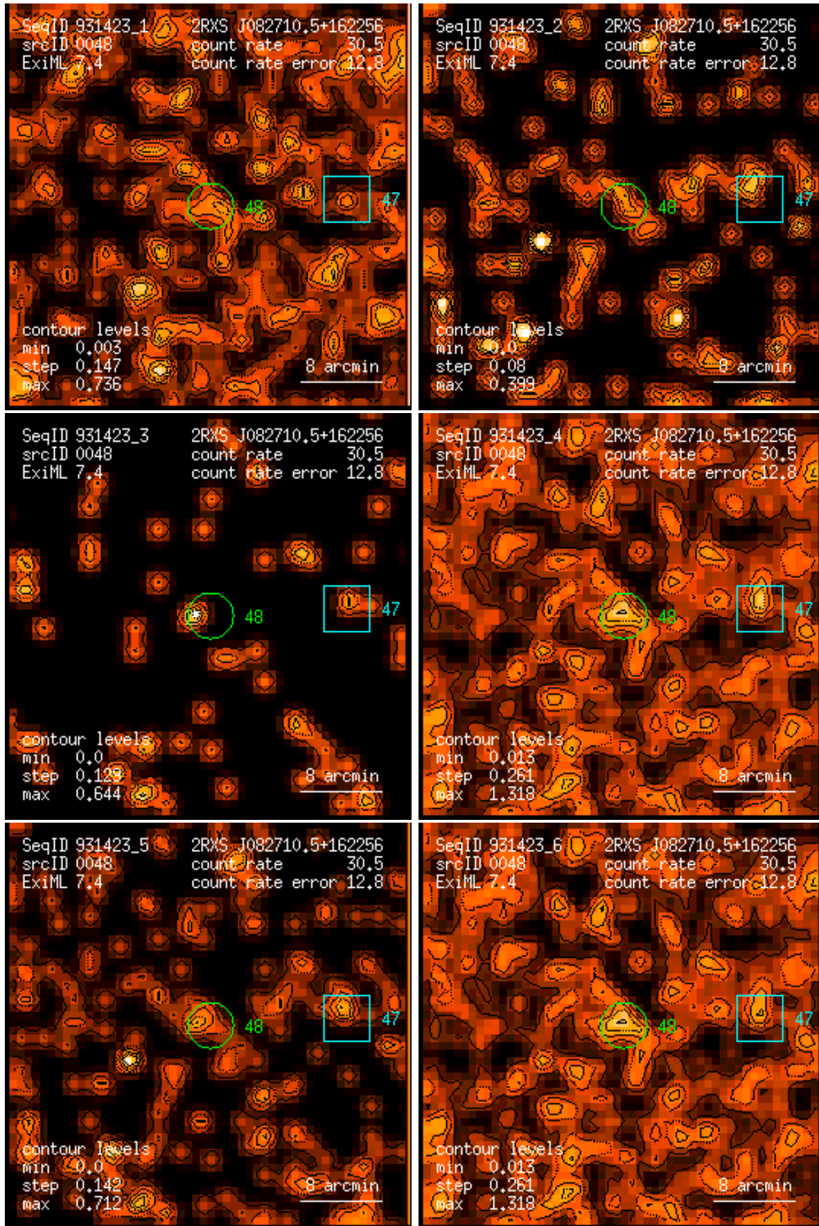
Figure 48: RASS 931423: detection 0048: band rate images, Gaussian filter: (1) PSPC channels 11 – 41, (2) 52 – 90, (3) 91 – 201, (4) 11 – 235, (5) 52 – 201, (6) 11 – 201. Broad band rates in counts/ks. Band rate contour levels in counts/ks/arcmin 2 .
