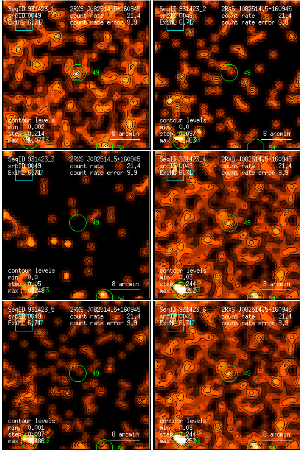
Figure 49: RASS 931423: detection 0049: band rate images, Gaussian filter: (1) PSPC channels 11 – 41, (2) 52 – 90, (3) 91 – 201, (4) 11 – 235, (5) 52 – 201, (6) 11 – 201. Broad band rates in counts/ks. Band rate contour levels in counts/ks/arcmin 2 .
