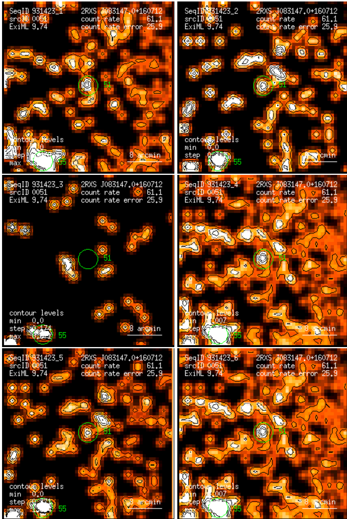
Figure 51: RASS 931423: detection 0051: band rate images, Gaussian filter: (1) PSPC channels 11 – 41, (2) 52 – 90, (3) 91 – 201, (4) 11 – 235, (5) 52 – 201, (6) 11 – 201. Broad band rates in counts/ks. Band rate contour levels in counts/ks/arcmin 2 .
