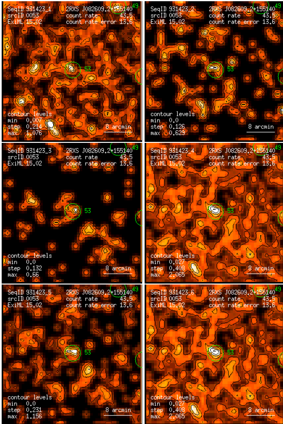
Figure 53: RASS 931423: detection 0053: band rate images, Gaussian filter: (1) PSPC channels 11 – 41, (2) 52 – 90, (3) 91 – 201, (4) 11 – 235, (5) 52 – 201, (6) 11 – 201. Broad band rates in counts/ks. Band rate contour levels in counts/ks/arcmin 2 .
