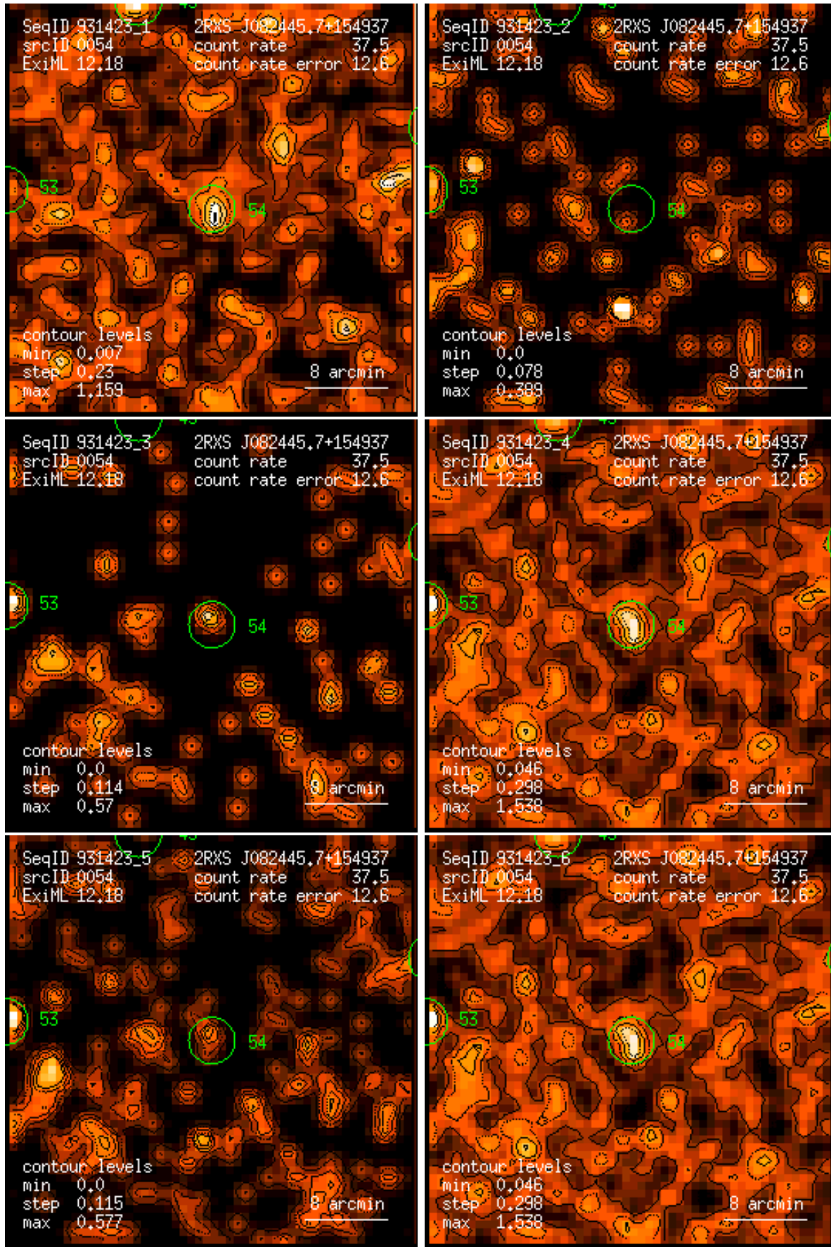
Figure 54: RASS 931423: detection 0054: band rate images, Gaussian filter: (1) PSPC channels 11 – 41, (2) 52 – 90, (3) 91 – 201, (4) 11 – 235, (5) 52 – 201, (6) 11 – 201. Broad band rates in counts/ks. Band rate contour levels in counts/ks/arcmin 2 .
