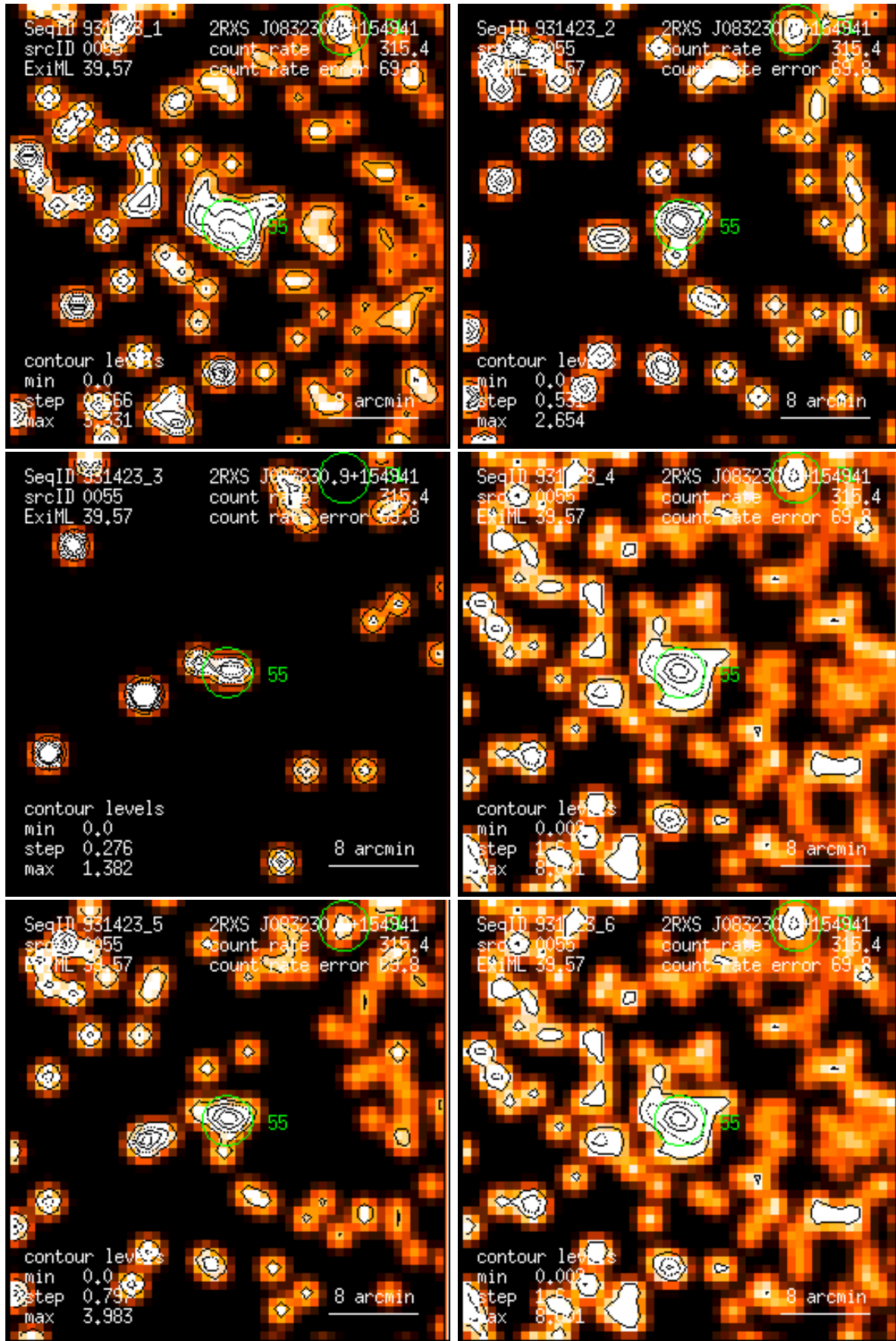
Figure 55: RASS 931423: detection 0055: band rate images, Gaussian filter: (1) PSPC channels 11 – 41, (2) 52 – 90, (3) 91 – 201, (4) 11 – 235, (5) 52 – 201, (6) 11 – 201. Broad band rates in counts/ks. Band rate contour levels in counts/ks/arcmin 2 .
