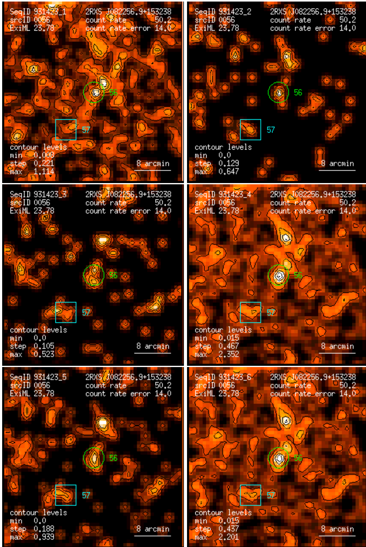
Figure 56: RASS 931423: detection 0056: band rate images, Gaussian filter: (1) PSPC channels 11 – 41, (2) 52 – 90, (3) 91 – 201, (4) 11 – 235, (5) 52 – 201, (6) 11 – 201. Broad band rates in counts/ks. Band rate contour levels in counts/ks/arcmin 2 .
