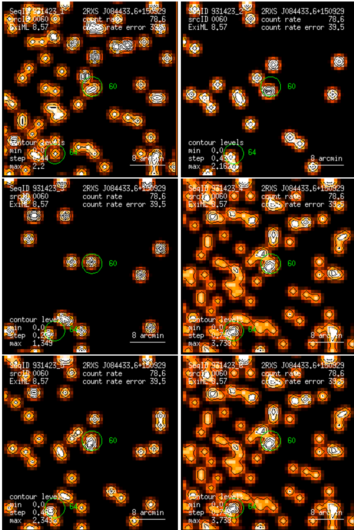
Figure 60: RASS 931423: detection 0060: band rate images, Gaussian filter: (1) PSPC channels 11 – 41, (2) 52 – 90, (3) 91 – 201, (4) 11 – 235, (5) 52 – 201, (6) 11 – 201. Broad band rates in counts/ks. Band rate contour levels in counts/ks/arcmin 2 .
