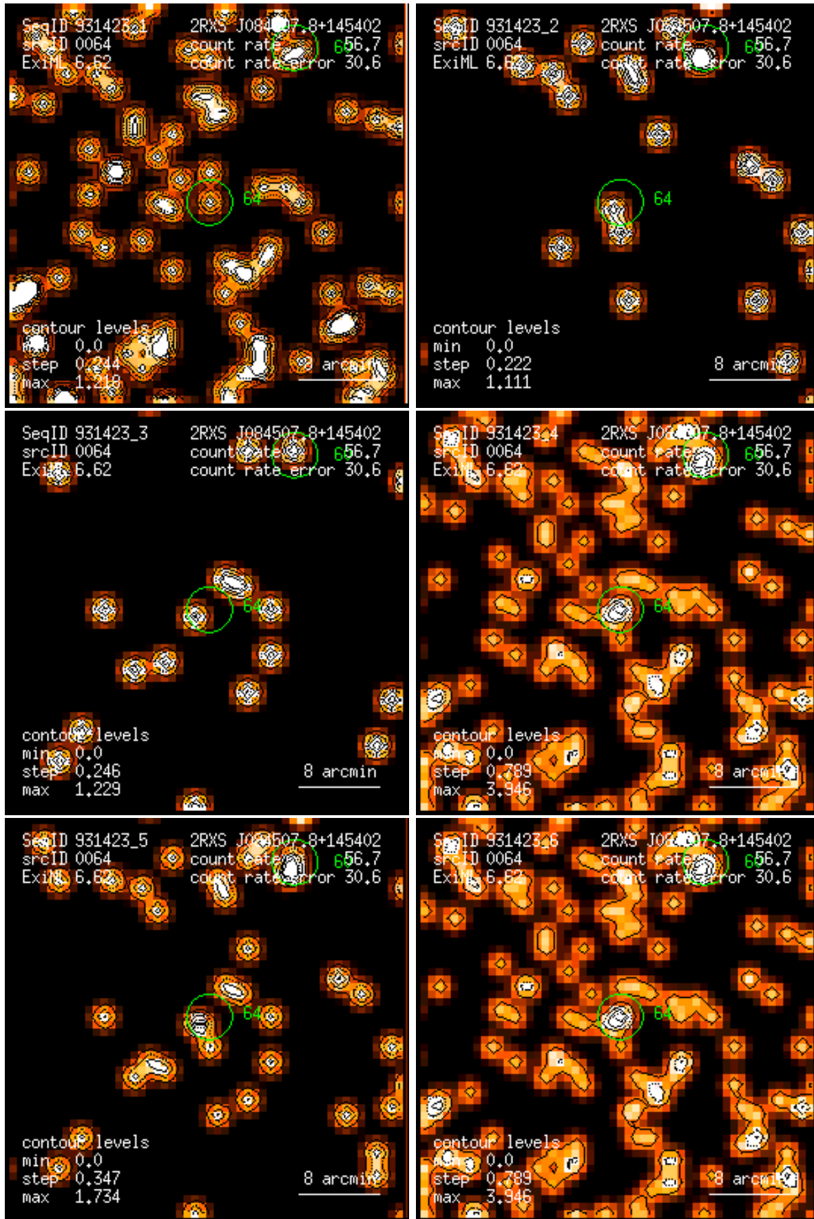
Figure 64: RASS 931423: detection 0064: band rate images, Gaussian filter: (1) PSPC channels 11 – 41, (2) 52 – 90, (3) 91 – 201, (4) 11 – 235, (5) 52 – 201, (6) 11 – 201. Broad band rates in counts/ks. Band rate contour levels in counts/ks/arcmin 2 .
