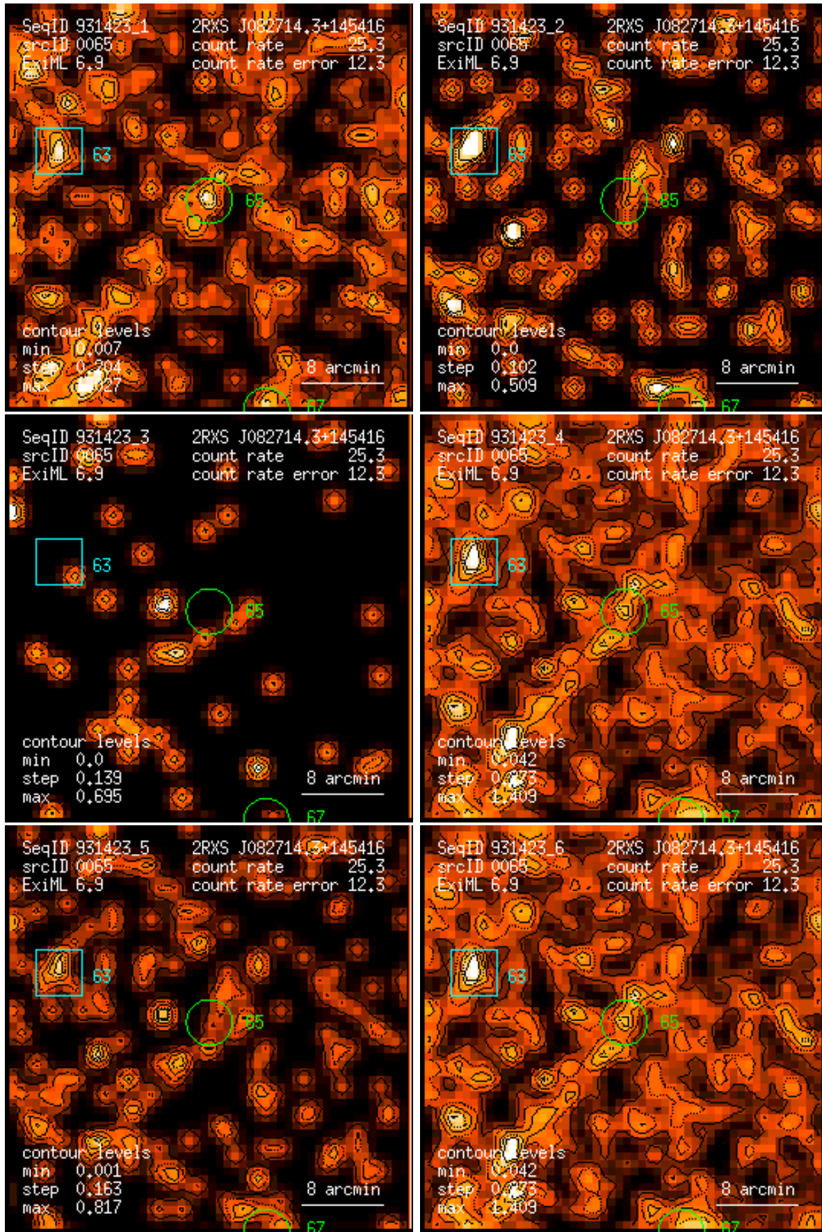
Figure 65: RASS 931423: detection 0065: band rate images, Gaussian filter: (1) PSPC channels 11 – 41, (2) 52 – 90, (3) 91 – 201, (4) 11 – 235, (5) 52 – 201, (6) 11 – 201. Broad band rates in counts/ks. Band rate contour levels in counts/ks/arcmin 2 .
