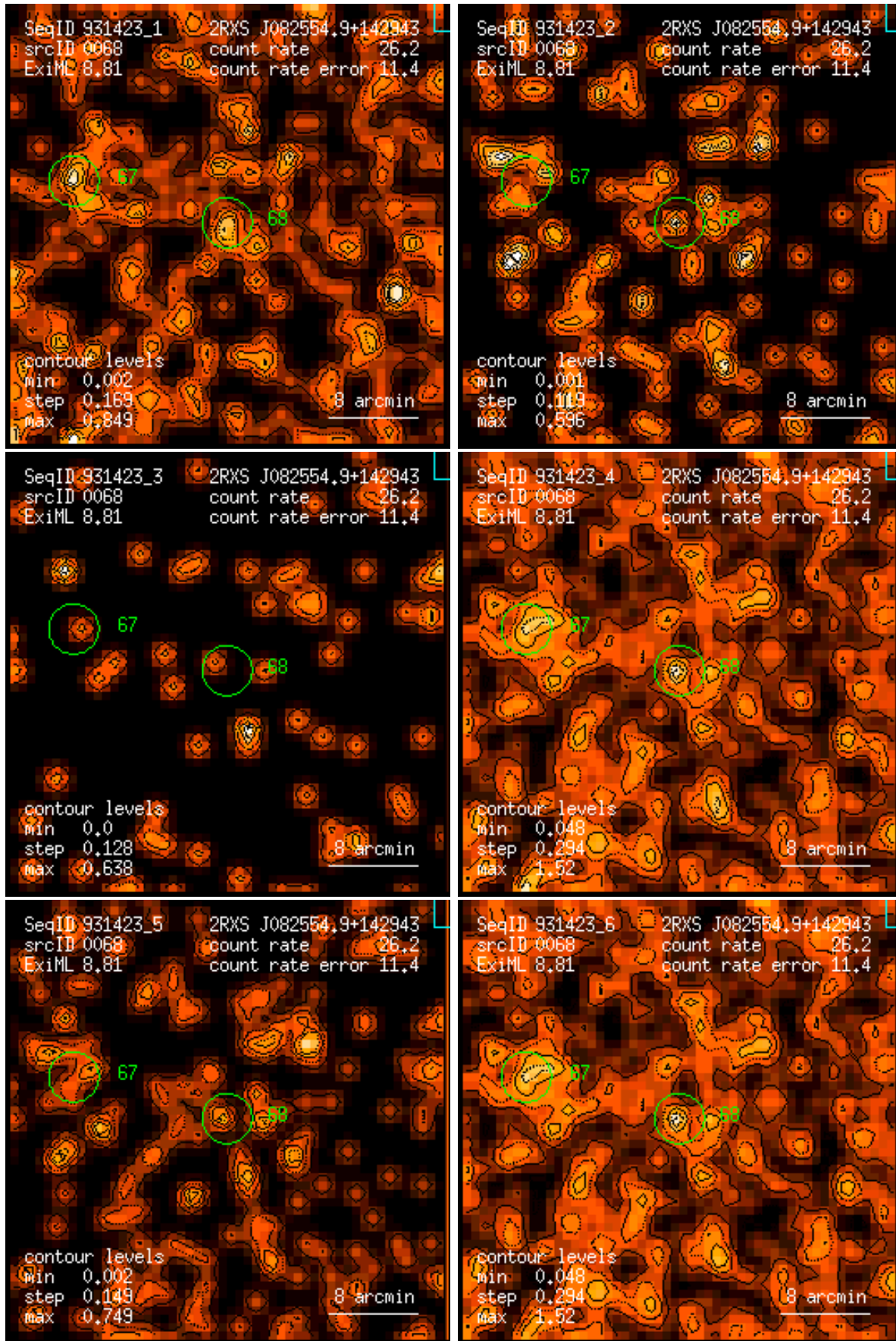
Figure 68: RASS 931423: detection 0068: band rate images, Gaussian filter: (1) PSPC channels 11 – 41, (2) 52 – 90, (3) 91 – 201, (4) 11 – 235, (5) 52 – 201, (6) 11 – 201. Broad band rates in counts/ks. Band rate contour levels in counts/ks/arcmin 2 .
