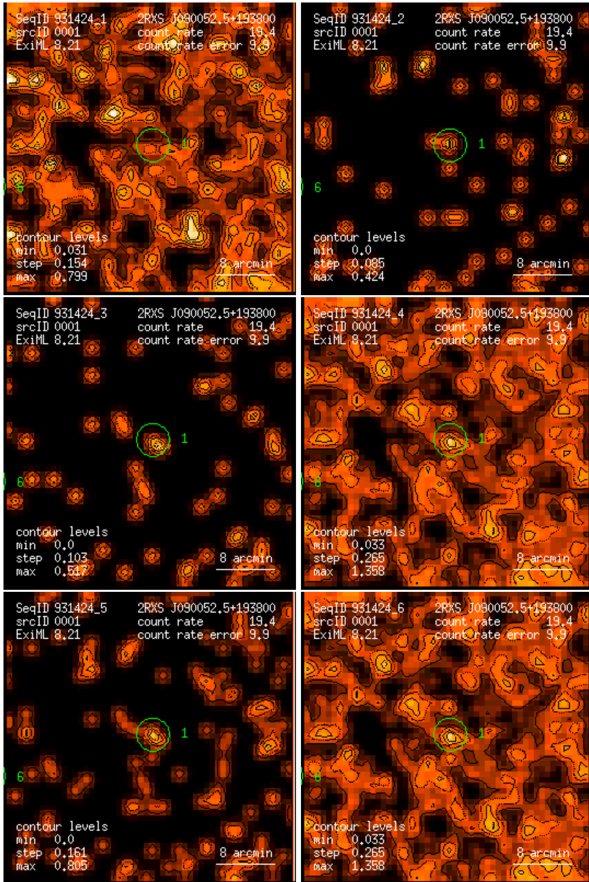
Figure 1: RASS 931424: detection 0001: band rate images, Gaussian filter: (1) PSPC channels 11 – 41, (2) 52 – 90, (3) 91 – 201, (4) 11 – 235, (5) 52 – 201, (6) 11 – 201. Broad band rates in counts/ks. Band rate contour levels in counts/ks/arcmin 2 .
