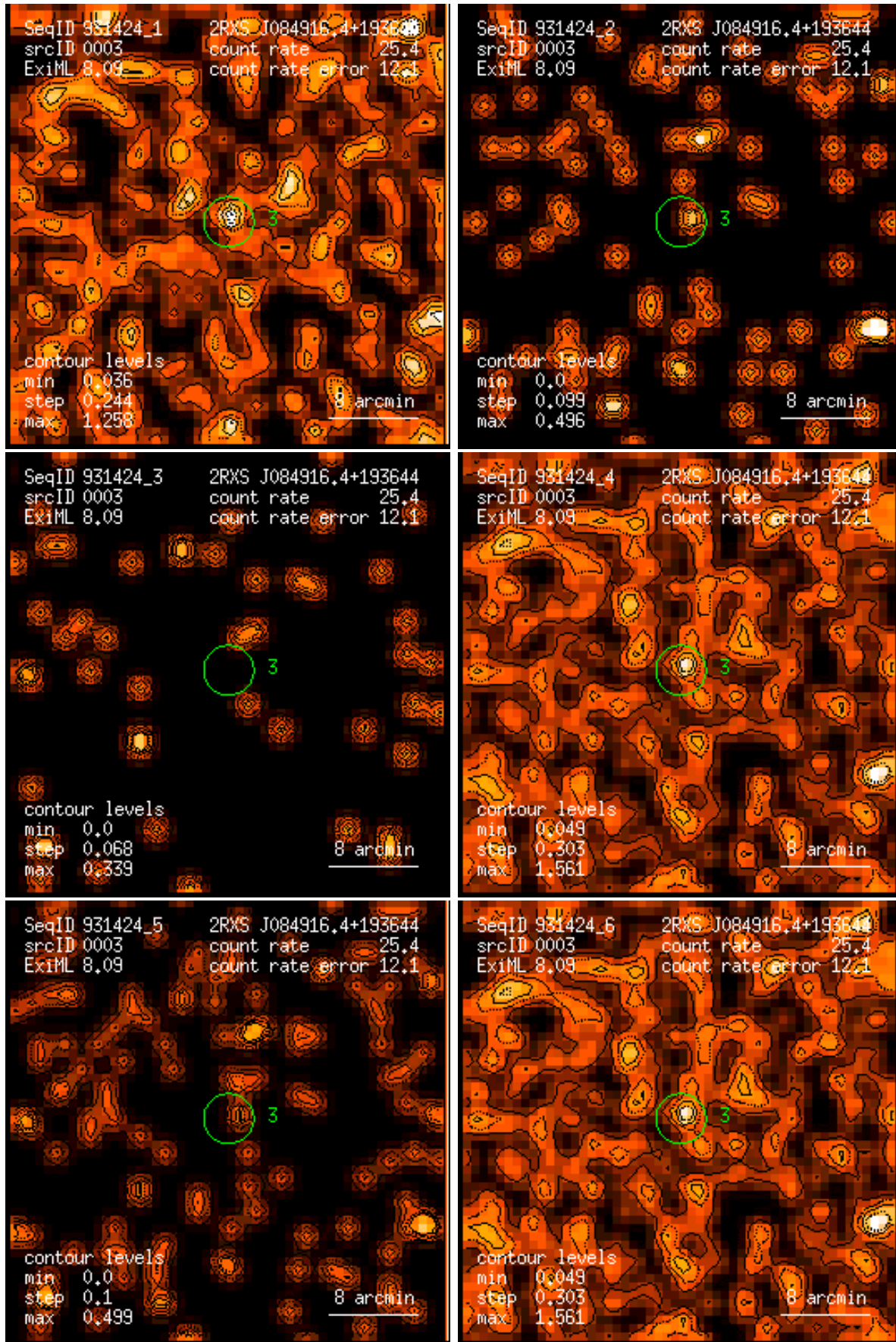
Figure 3: RASS 931424: detection 0003: band rate images, Gaussian filter: (1) PSPC channels 11 – 41, (2) 52 – 90, (3) 91 – 201, (4) 11 – 235, (5) 52 – 201, (6) 11 – 201. Broad band rates in counts/ks. Band rate contour levels in counts/ks/arcmin 2 .
