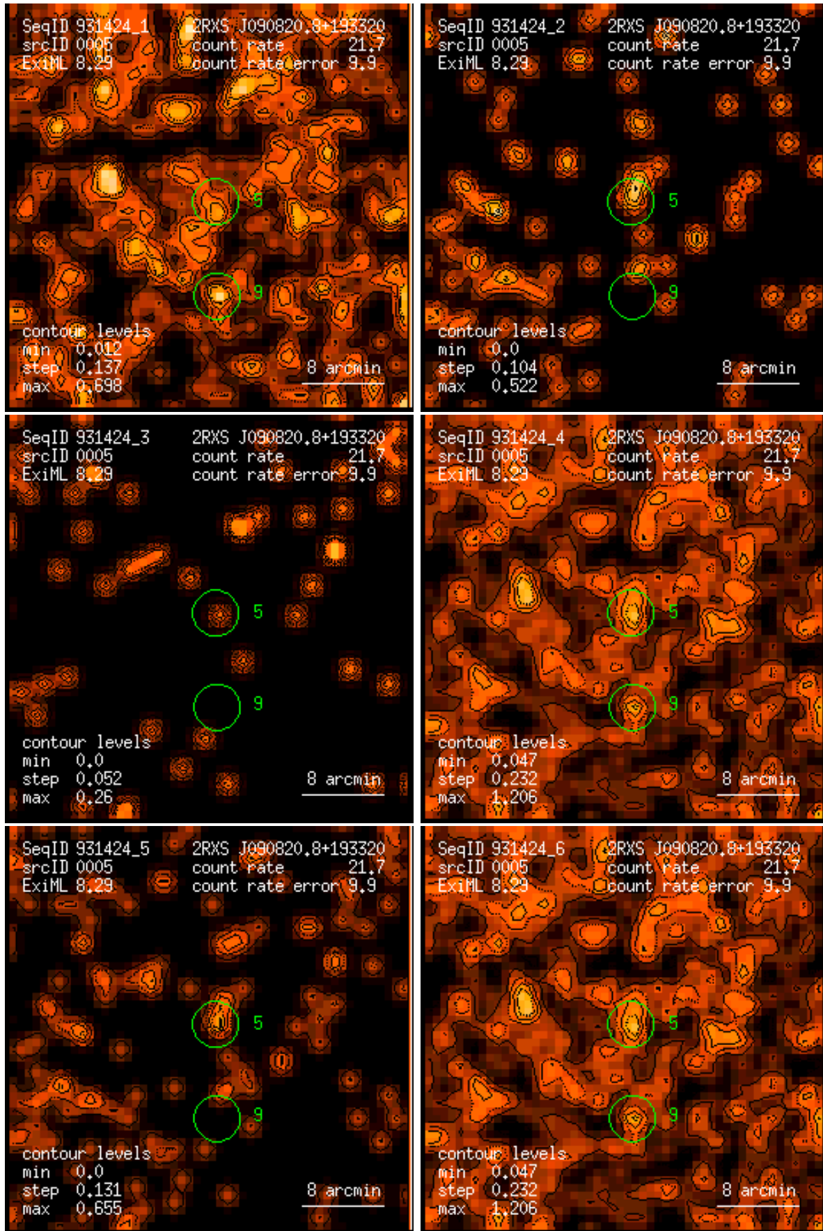
Figure 5: RASS 931424: detection 0005: band rate images, Gaussian filter: (1) PSPC channels 11 – 41, (2) 52 – 90, (3) 91 – 201, (4) 11 – 235, (5) 52 – 201, (6) 11 – 201. Broad band rates in counts/ks. Band rate contour levels in counts/ks/arcmin 2 .
