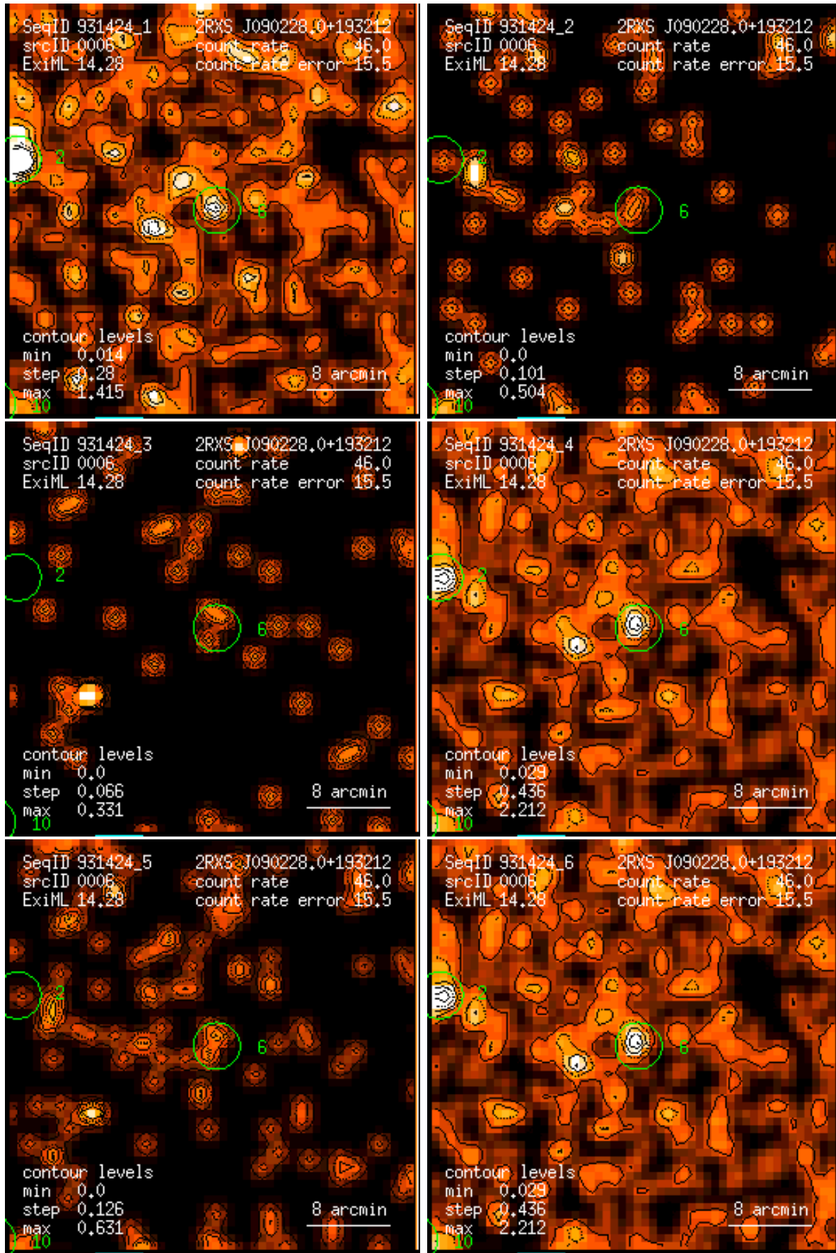
Figure 6: RASS 931424: detection 0006: band rate images, Gaussian filter: (1) PSPC channels 11 – 41, (2) 52 – 90, (3) 91 – 201, (4) 11 – 235, (5) 52 – 201, (6) 11 – 201. Broad band rates in counts/ks. Band rate contour levels in counts/ks/arcmin 2 .
