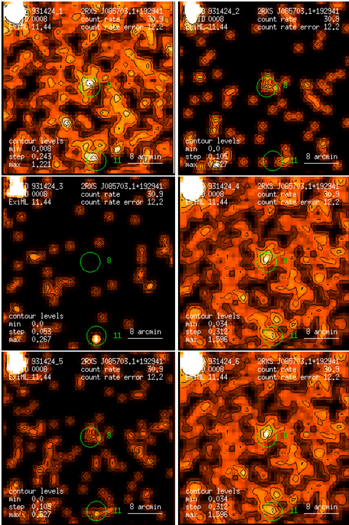
Figure 8: RASS 931424: detection 0008: band rate images, Gaussian filter: (1) PSPC channels 11 – 41, (2) 52 – 90, (3) 91 – 201, (4) 11 – 235, (5) 52 – 201, (6) 11 – 201. Broad band rates in counts/ks. Band rate contour levels in counts/ks/arcmin 2 .
