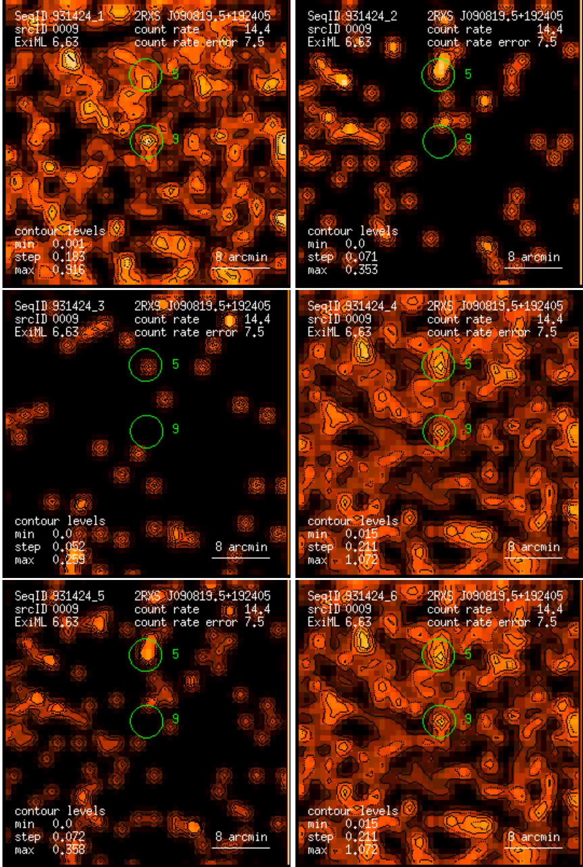
Figure 9: RASS 931424: detection 0009: band rate images, Gaussian filter: (1) PSPC channels 11 – 41, (2) 52 – 90, (3) 91 – 201, (4) 11 – 235, (5) 52 – 201, (6) 11 – 201. Broad band rates in counts/ks. Band rate contour levels in counts/ks/arcmin 2 .
