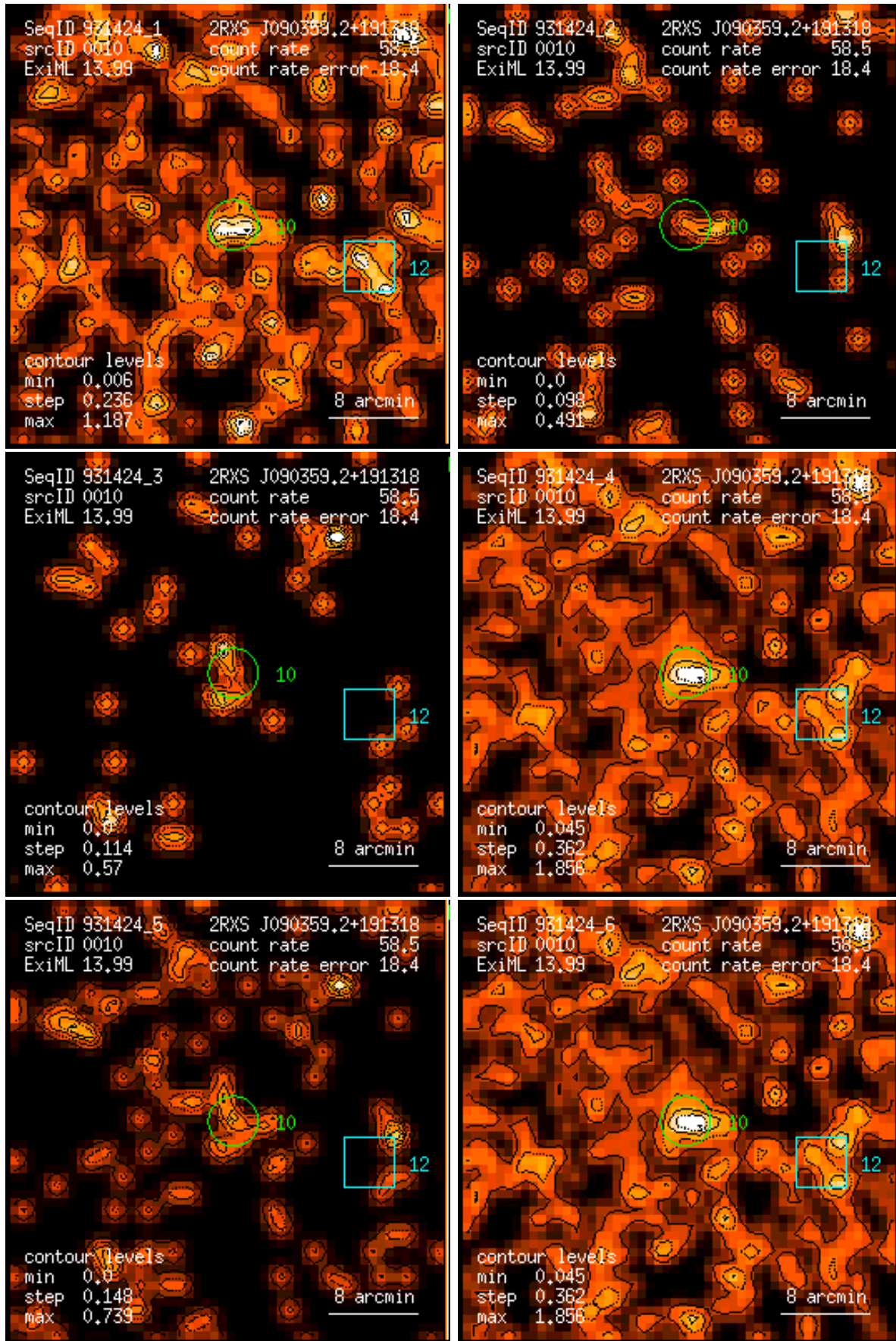
Figure 10: RASS 931424: detection 0010: band rate images, Gaussian filter: (1) PSPC channels 11 – 41, (2) 52 – 90, (3) 91 – 201, (4) 11 – 235, (5) 52 – 201, (6) 11 – 201. Broad band rates in counts/ks. Band rate contour levels in counts/ks/arcmin 2 .
