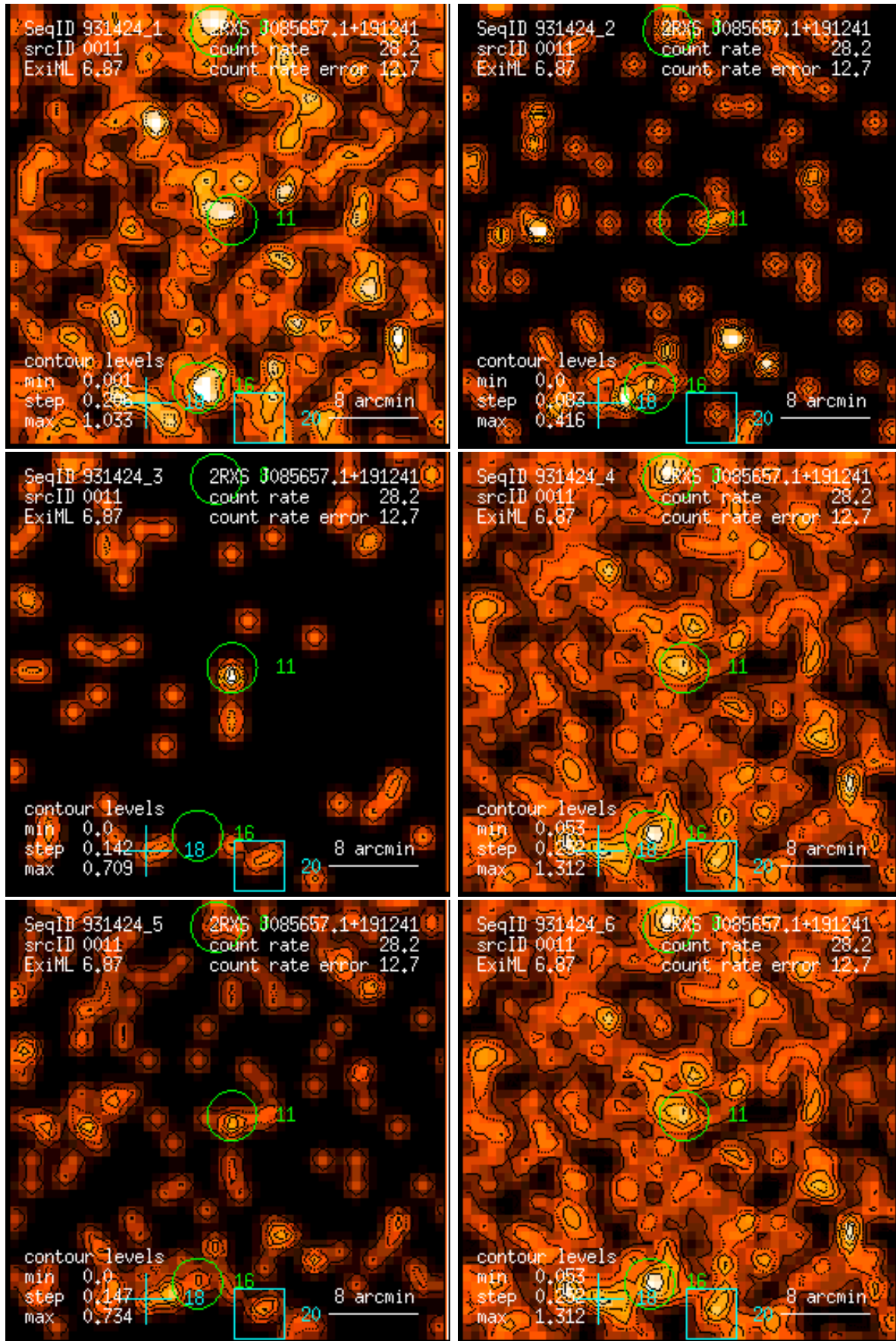
Figure 11: RASS 931424: detection 0011: band rate images, Gaussian filter: (1) PSPC channels 11 – 41, (2) 52 – 90, (3) 91 – 201, (4) 11 – 235, (5) 52 – 201, (6) 11 – 201. Broad band rates in counts/ks. Band rate contour levels in counts/ks/arcmin 2 .
