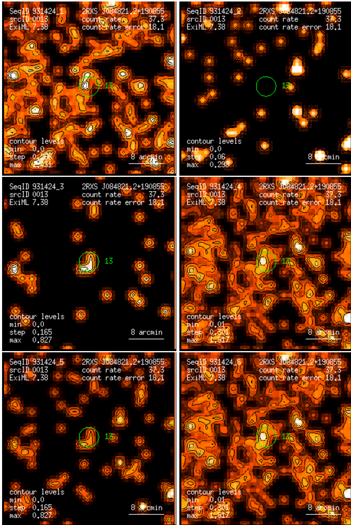
Figure 13: RASS 931424: detection 0013: band rate images, Gaussian filter: (1) PSPC channels 11 – 41, (2) 52 – 90, (3) 91 – 201, (4) 11 – 235, (5) 52 – 201, (6) 11 – 201. Broad band rates in counts/ks. Band rate contour levels in counts/ks/arcmin 2 .
