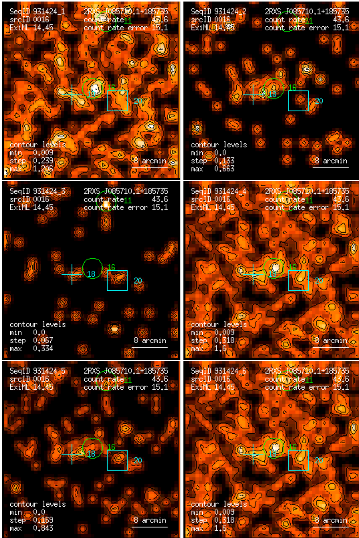
Figure 16: RASS 931424: detection 0016: band rate images, Gaussian filter: (1) PSPC channels 11 – 41, (2) 52 – 90, (3) 91 – 201, (4) 11 – 235, (5) 52 – 201, (6) 11 – 201. Broad band rates in counts/ks. Band rate contour levels in counts/ks/arcmin 2 .
