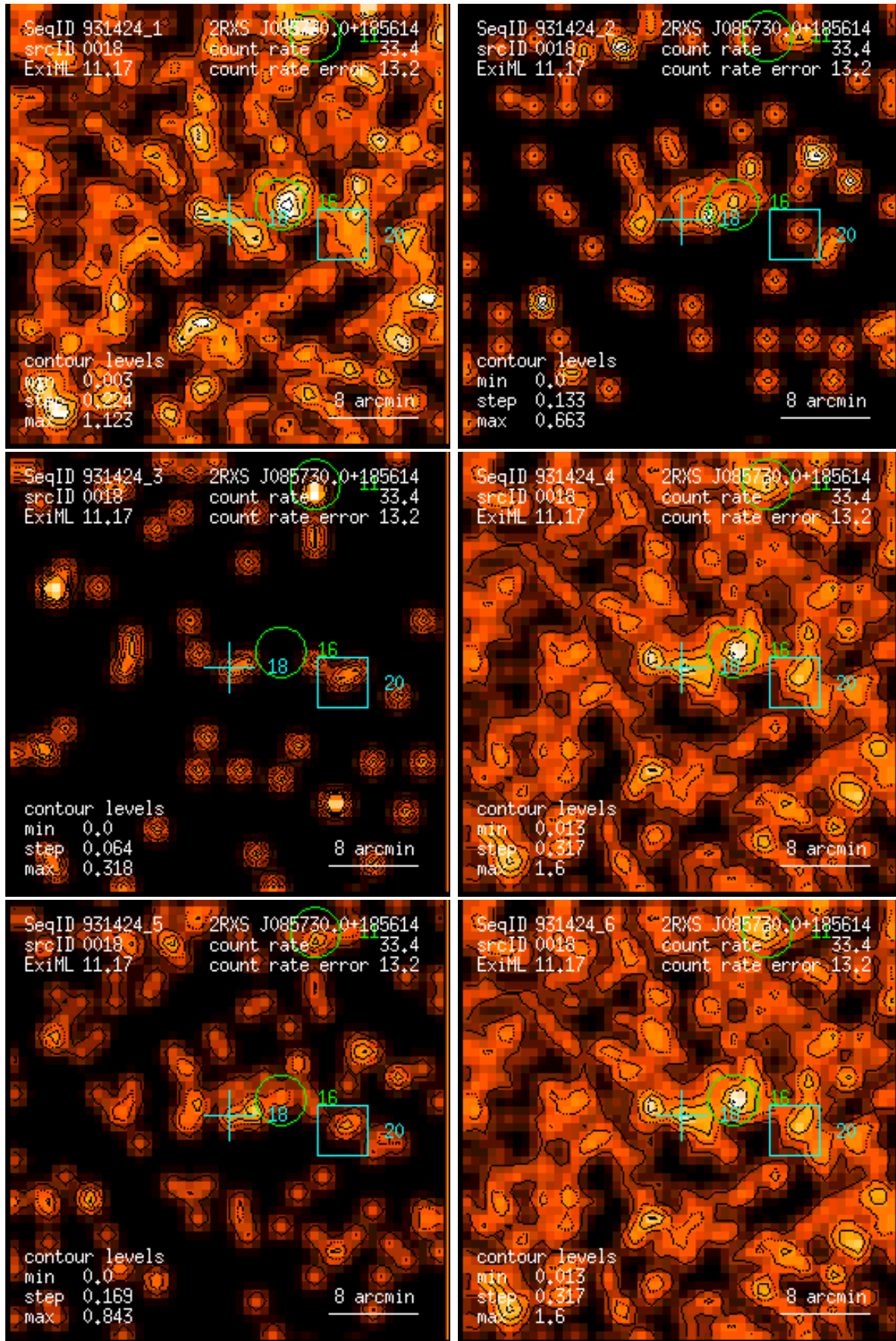
Figure 18: RASS 931424: detection 0018: band rate images, Gaussian filter: (1) PSPC channels 11 – 41, (2) 52 – 90, (3) 91 – 201, (4) 11 – 235, (5) 52 – 201, (6) 11 – 201. Broad band rates in counts/ks. Band rate contour levels in counts/ks/arcmin 2 .
