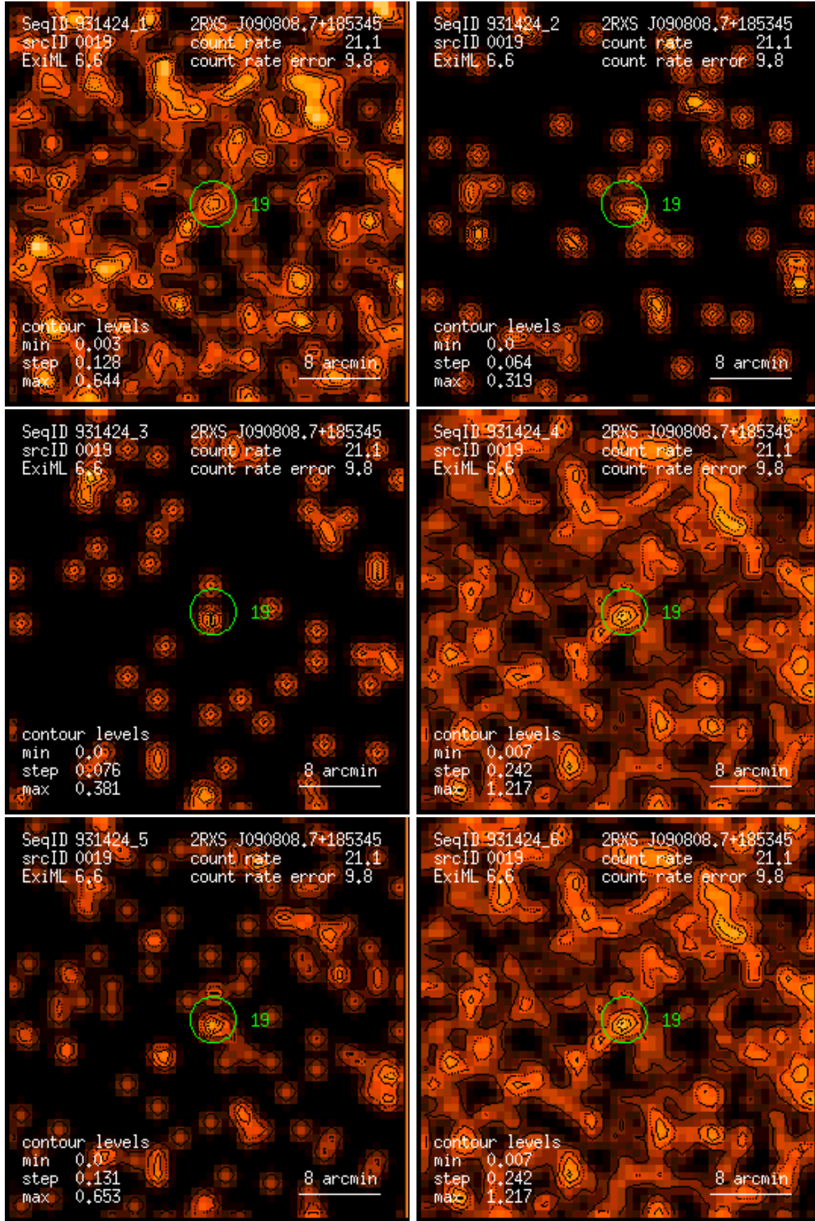
Figure 19: RASS 931424: detection 0019: band rate images, Gaussian filter: (1) PSPC channels 11 – 41, (2) 52 – 90, (3) 91 – 201, (4) 11 – 235, (5) 52 – 201, (6) 11 – 201. Broad band rates in counts/ks. Band rate contour levels in counts/ks/arcmin 2 .
