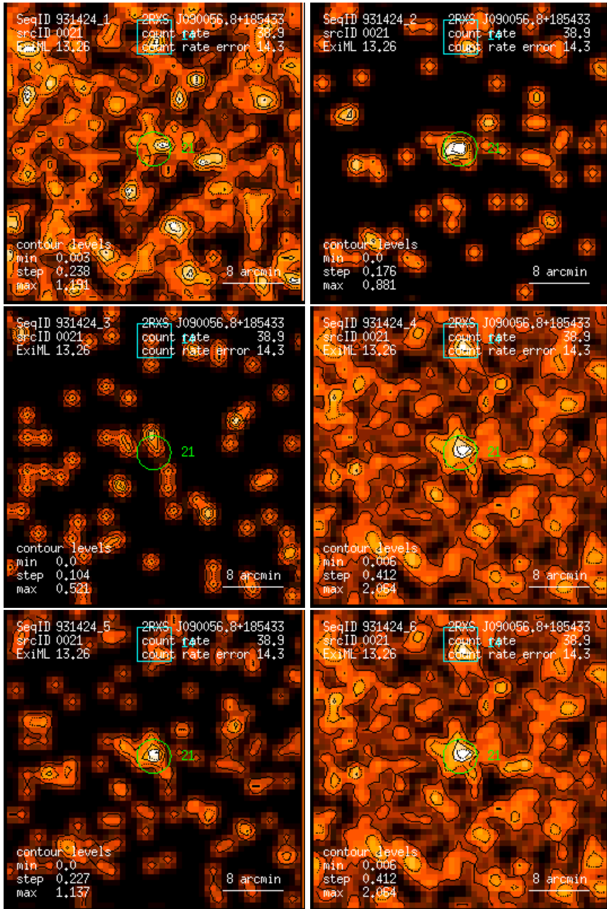
Figure 21: RASS 931424: detection 0021: band rate images, Gaussian filter: (1) PSPC channels 11 – 41, (2) 52 – 90, (3) 91 – 201, (4) 11 – 235, (5) 52 – 201, (6) 11 – 201. Broad band rates in counts/ks. Band rate contour levels in counts/ks/arcmin 2 .
