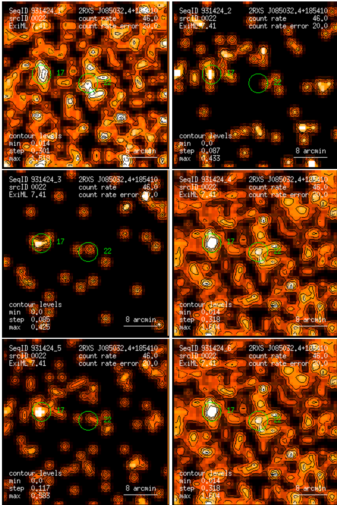
Figure 22: RASS 931424: detection 0022: band rate images, Gaussian filter: (1) PSPC channels 11 – 41, (2) 52 – 90, (3) 91 – 201, (4) 11 – 235, (5) 52 – 201, (6) 11 – 201. Broad band rates in counts/ks. Band rate contour levels in counts/ks/arcmin 2 .
