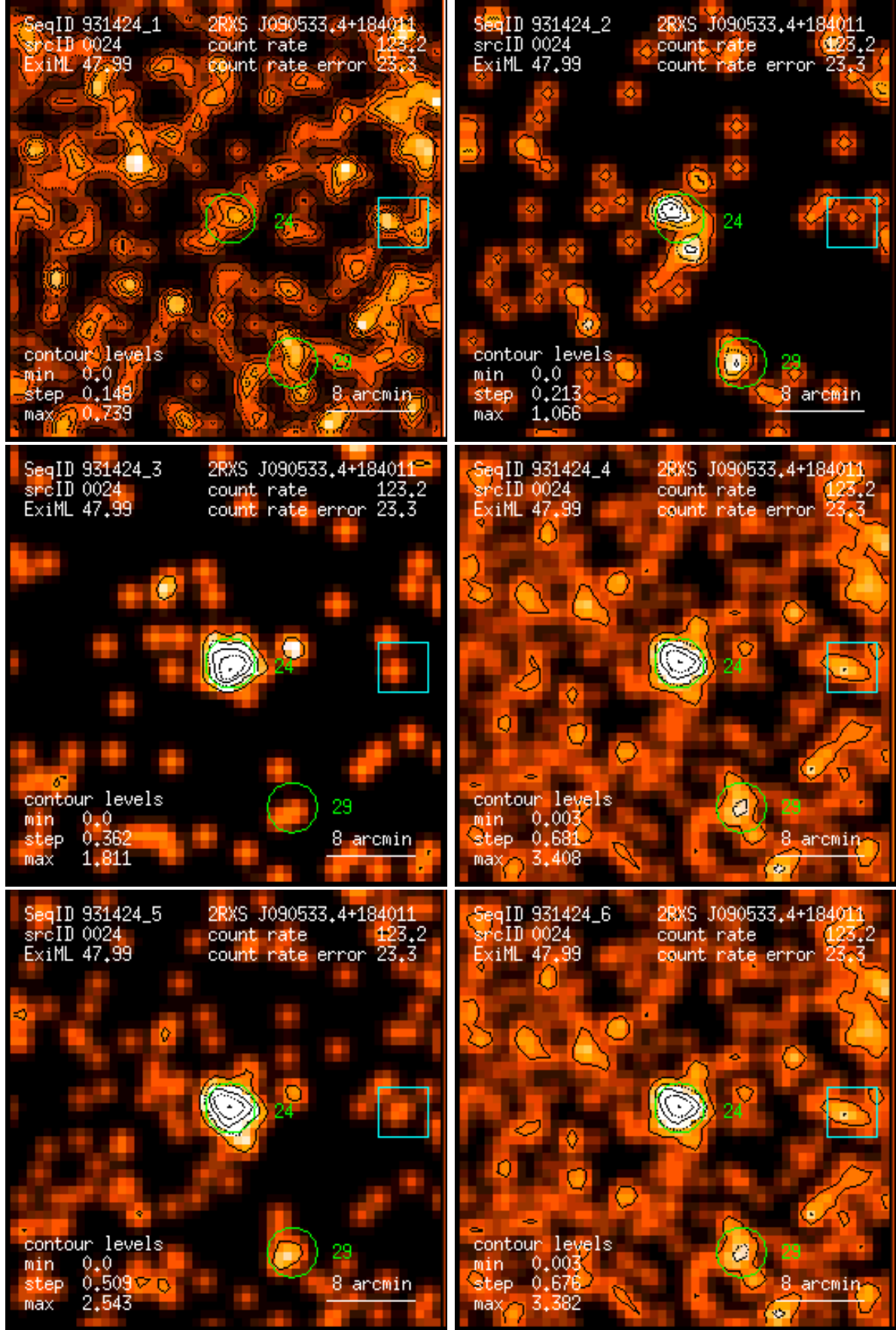
Figure 24: RASS 931424: detection 0024: band rate images, Gaussian filter: (1) PSPC channels 11 – 41, (2) 52 – 90, (3) 91 – 201, (4) 11 – 235, (5) 52 – 201, (6) 11 – 201. Broad band rates in counts/ks. Band rate contour levels in counts/ks/arcmin 2 .
