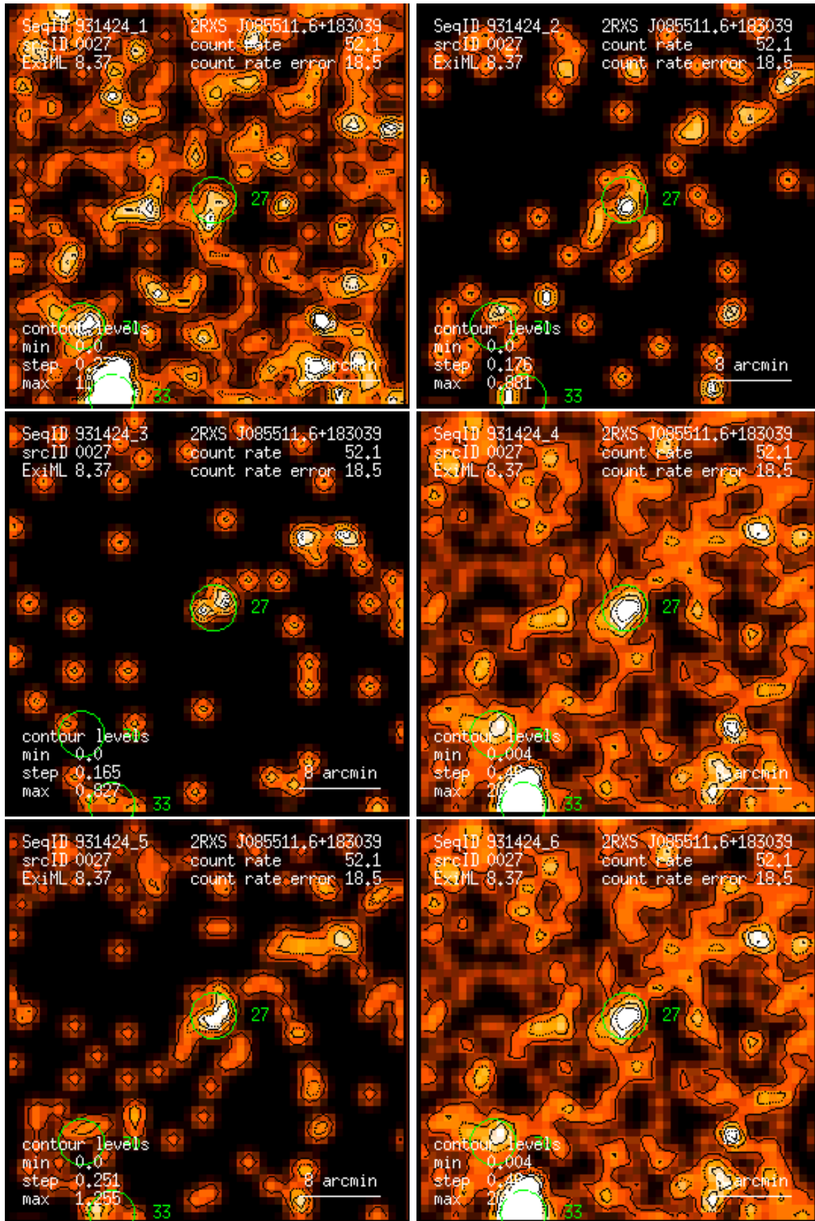
Figure 27: RASS 931424: detection 0027: band rate images, Gaussian filter: (1) PSPC channels 11 – 41, (2) 52 – 90, (3) 91 – 201, (4) 11 – 235, (5) 52 – 201, (6) 11 – 201. Broad band rates in counts/ks. Band rate contour levels in counts/ks/arcmin 2 .
