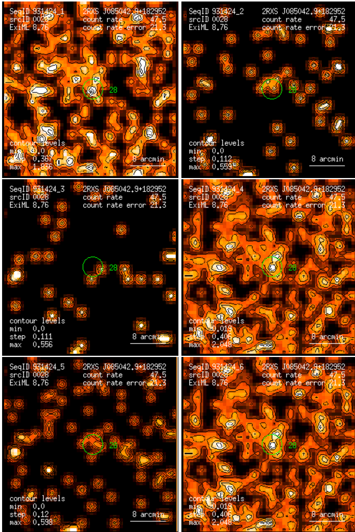
Figure 28: RASS 931424: detection 0028: band rate images, Gaussian filter: (1) PSPC channels 11 – 41, (2) 52 – 90, (3) 91 – 201, (4) 11 – 235, (5) 52 – 201, (6) 11 – 201. Broad band rates in counts/ks. Band rate contour levels in counts/ks/arcmin 2 .
