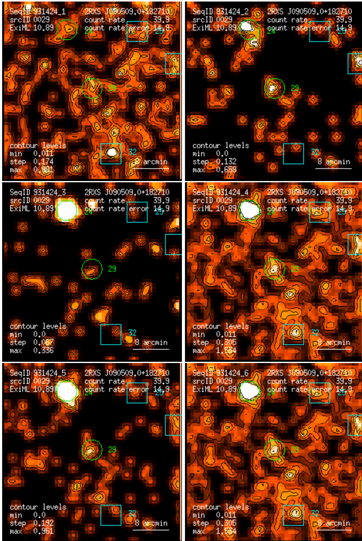
Figure 29: RASS 931424: detection 0029: band rate images, Gaussian filter: (1) PSPC channels 11 – 41, (2) 52 – 90, (3) 91 – 201, (4) 11 – 235, (5) 52 – 201, (6) 11 – 201. Broad band rates in counts/ks. Band rate contour levels in counts/ks/arcmin 2 .
