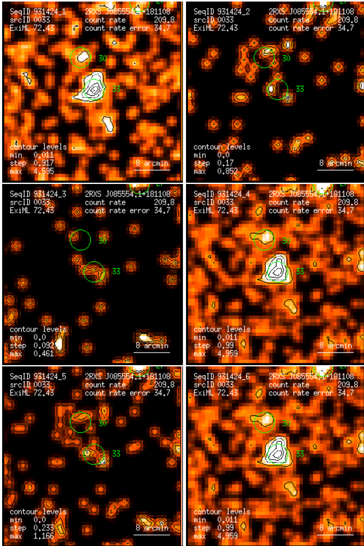
Figure 33: RASS 931424: detection 0033: band rate images, Gaussian filter: (1) PSPC channels 11 – 41, (2) 52 – 90, (3) 91 – 201, (4) 11 – 235, (5) 52 – 201, (6) 11 – 201. Broad band rates in counts/ks. Band rate contour levels in counts/ks/arcmin 2 .
