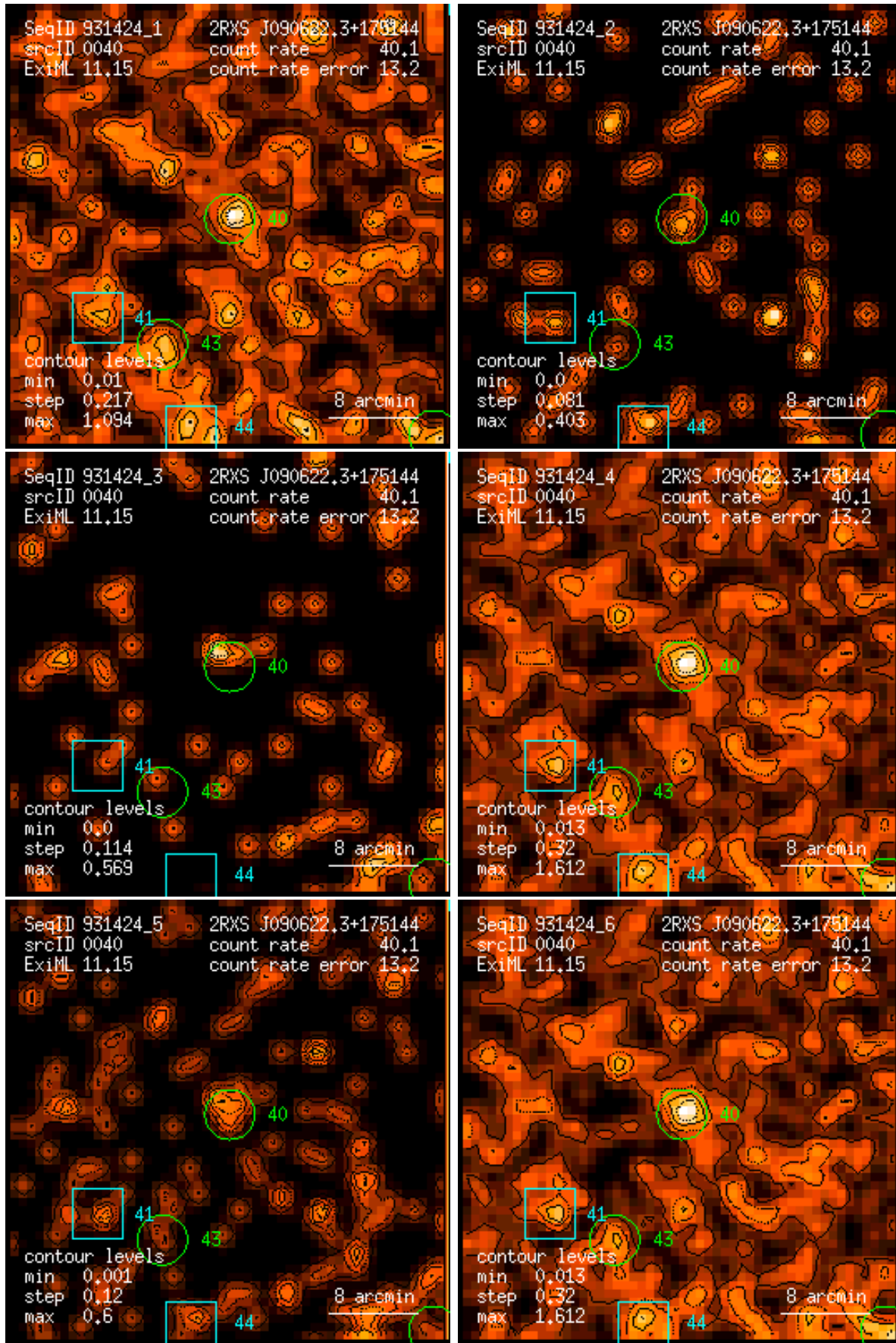
Figure 40: RASS 931424: detection 0040: band rate images, Gaussian filter: (1) PSPC channels 11 – 41, (2) 52 – 90, (3) 91 – 201, (4) 11 – 235, (5) 52 – 201, (6) 11 – 201. Broad band rates in counts/ks. Band rate contour levels in counts/ks/arcmin 2 .
