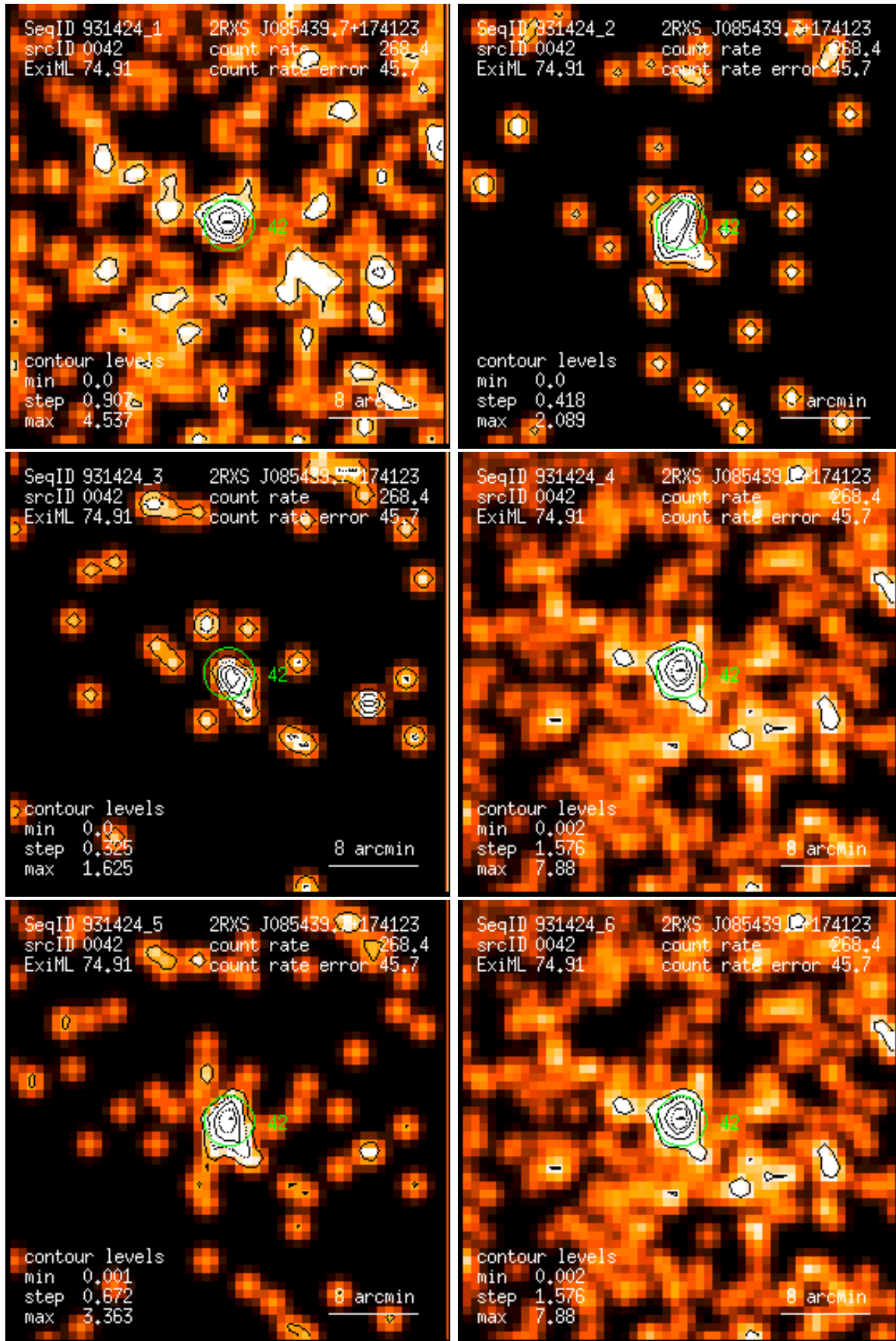
Figure 42: RASS 931424: detection 0042: band rate images, Gaussian filter: (1) PSPC channels 11 – 41, (2) 52 – 90, (3) 91 – 201, (4) 11 – 235, (5) 52 – 201, (6) 11 – 201. Broad band rates in counts/ks. Band rate contour levels in counts/ks/arcmin 2 .
