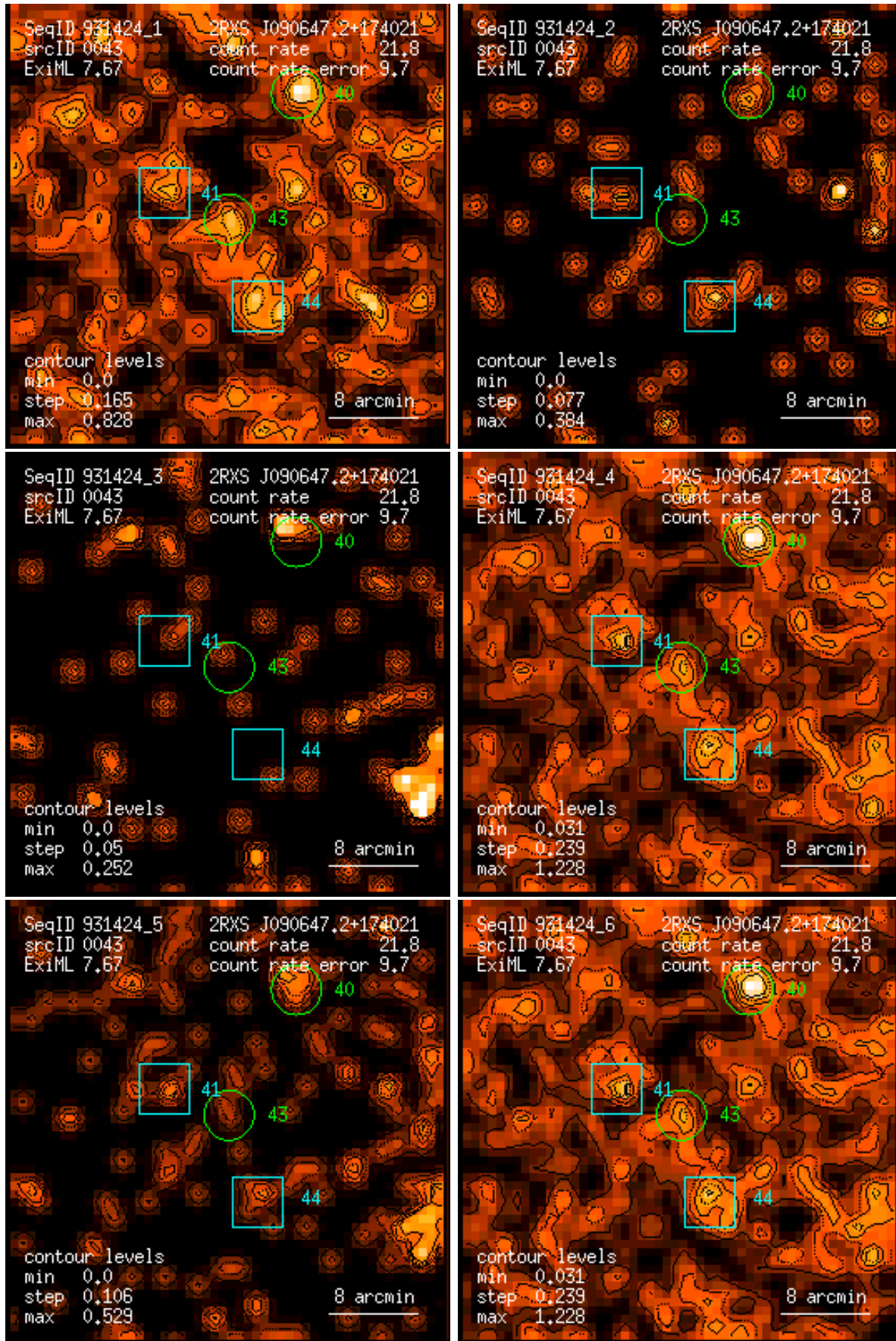
Figure 43: RASS 931424: detection 0043: band rate images, Gaussian filter: (1) PSPC channels 11 – 41, (2) 52 – 90, (3) 91 – 201, (4) 11 – 235, (5) 52 – 201, (6) 11 – 201. Broad band rates in counts/ks. Band rate contour levels in counts/ks/arcmin 2 .
