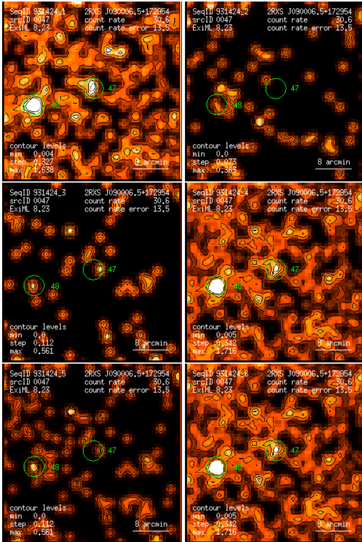
Figure 47: RASS 931424: detection 0047: band rate images, Gaussian filter: (1) PSPC channels 11 – 41, (2) 52 – 90, (3) 91 – 201, (4) 11 – 235, (5) 52 – 201, (6) 11 – 201. Broad band rates in counts/ks. Band rate contour levels in counts/ks/arcmin 2 .
