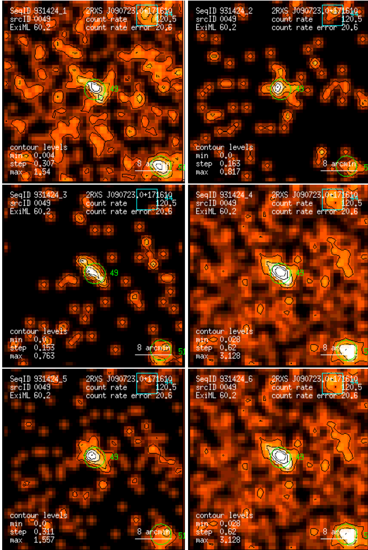
Figure 49: RASS 931424: detection 0049: band rate images, Gaussian filter: (1) PSPC channels 11 – 41, (2) 52 – 90, (3) 91 – 201, (4) 11 – 235, (5) 52 – 201, (6) 11 – 201. Broad band rates in counts/ks. Band rate contour levels in counts/ks/arcmin 2 .
