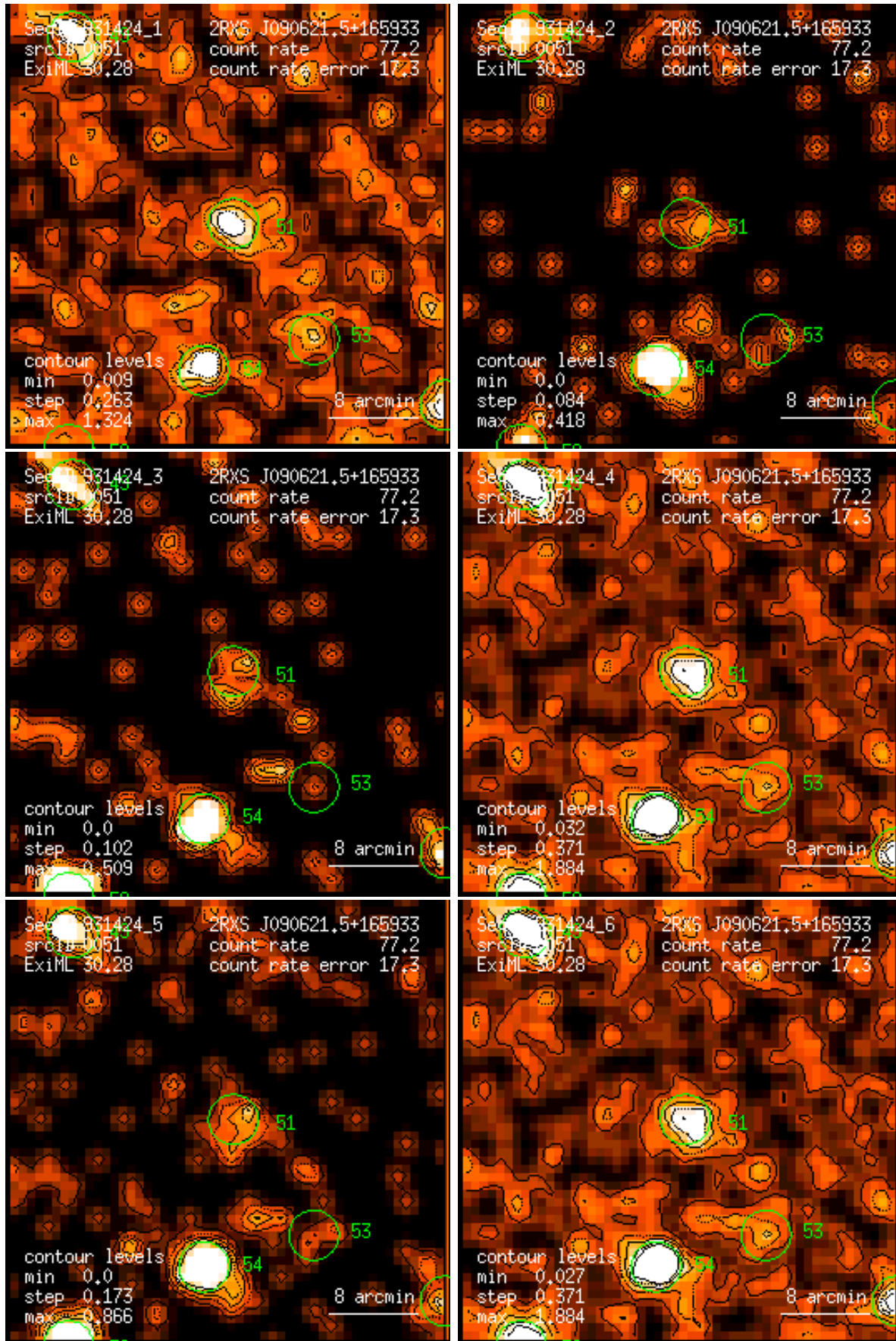
Figure 51: RASS 931424: detection 0051: band rate images, Gaussian filter: (1) PSPC channels 11 – 41, (2) 52 – 90, (3) 91 – 201, (4) 11 – 235, (5) 52 – 201, (6) 11 – 201. Broad band rates in counts/ks. Band rate contour levels in counts/ks/arcmin 2 .
