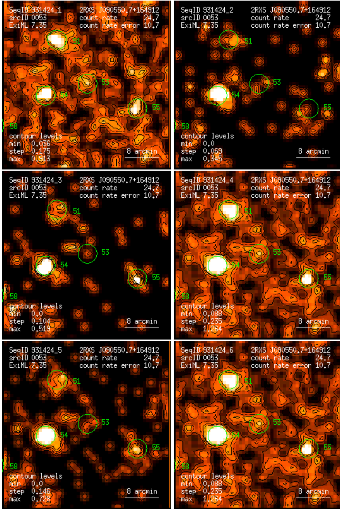
Figure 53: RASS 931424: detection 0053: band rate images, Gaussian filter: (1) PSPC channels 11 – 41, (2) 52 – 90, (3) 91 – 201, (4) 11 – 235, (5) 52 – 201, (6) 11 – 201. Broad band rates in counts/ks. Band rate contour levels in counts/ks/arcmin 2 .
