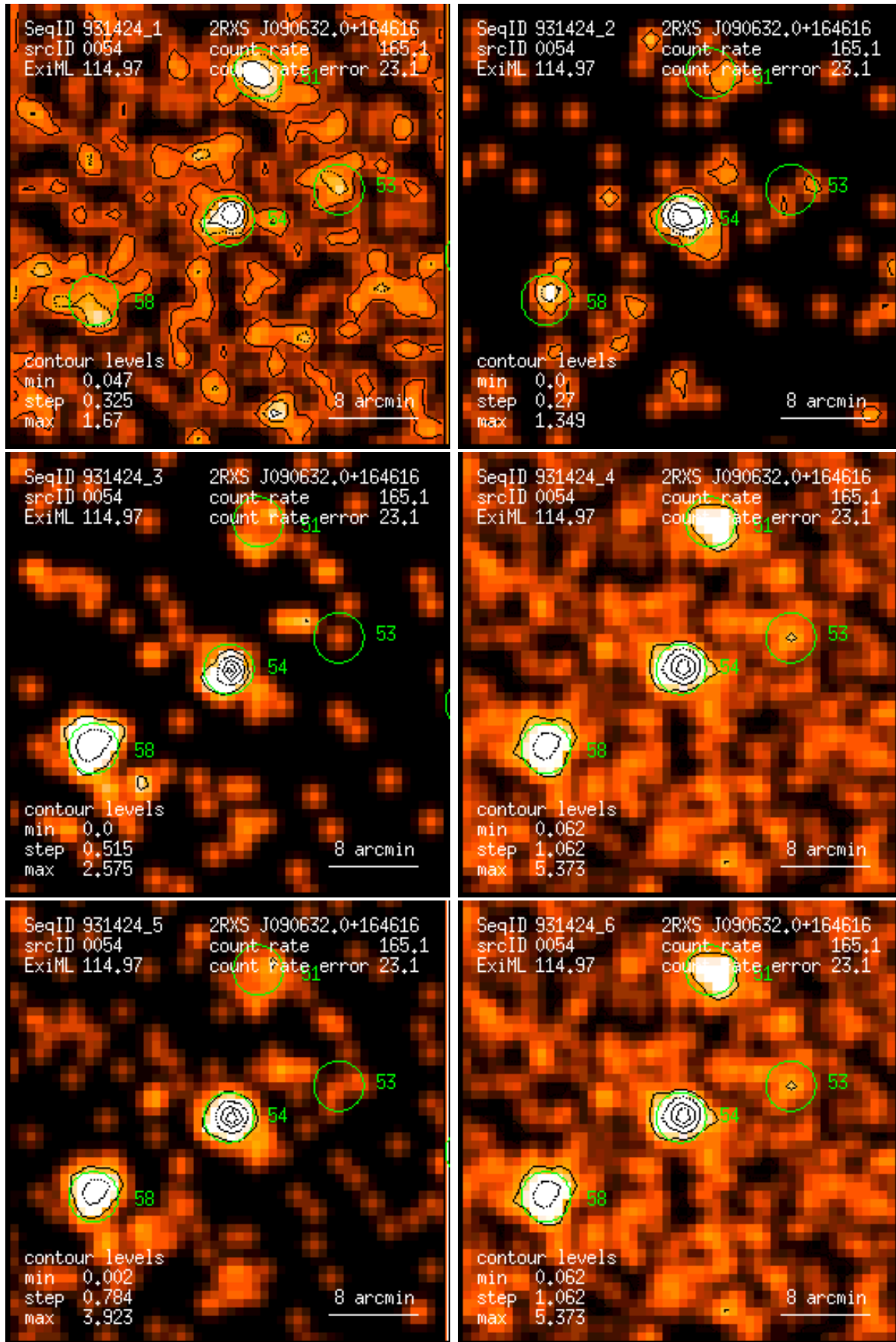
Figure 54: RASS 931424: detection 0054: band rate images, Gaussian filter: (1) PSPC channels 11 – 41, (2) 52 – 90, (3) 91 – 201, (4) 11 – 235, (5) 52 – 201, (6) 11 – 201. Broad band rates in counts/ks. Band rate contour levels in counts/ks/arcmin 2 .
