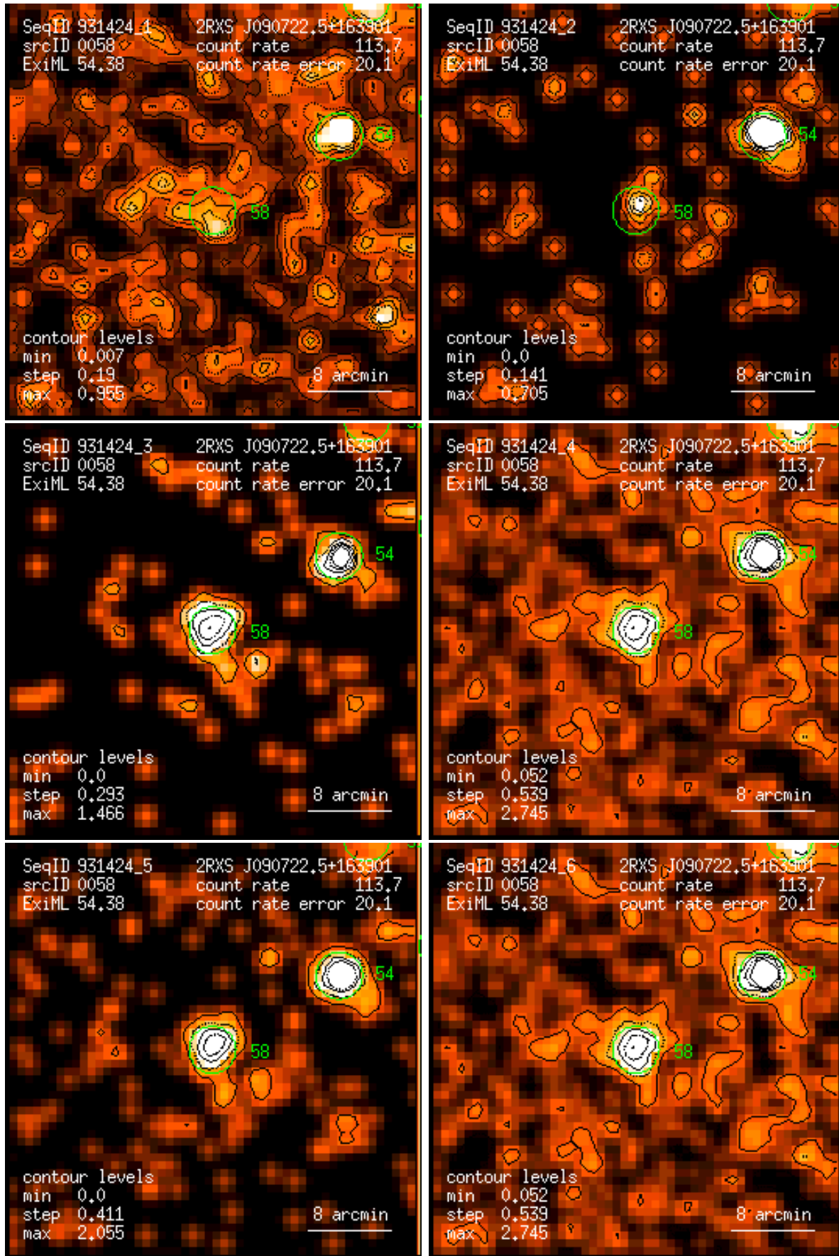
Figure 58: RASS 931424: detection 0058: band rate images, Gaussian filter: (1) PSPC channels 11 – 41, (2) 52 – 90, (3) 91 – 201, (4) 11 – 235, (5) 52 – 201, (6) 11 – 201. Broad band rates in counts/ks. Band rate contour levels in counts/ks/arcmin 2 .
