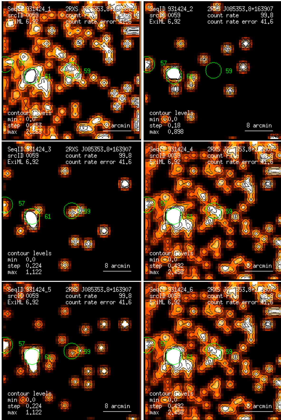
Figure 59: RASS 931424: detection 0059: band rate images, Gaussian filter: (1) PSPC channels 11 – 41, (2) 52 – 90, (3) 91 – 201, (4) 11 – 235, (5) 52 – 201, (6) 11 – 201. Broad band rates in counts/ks. Band rate contour levels in counts/ks/arcmin 2 .
