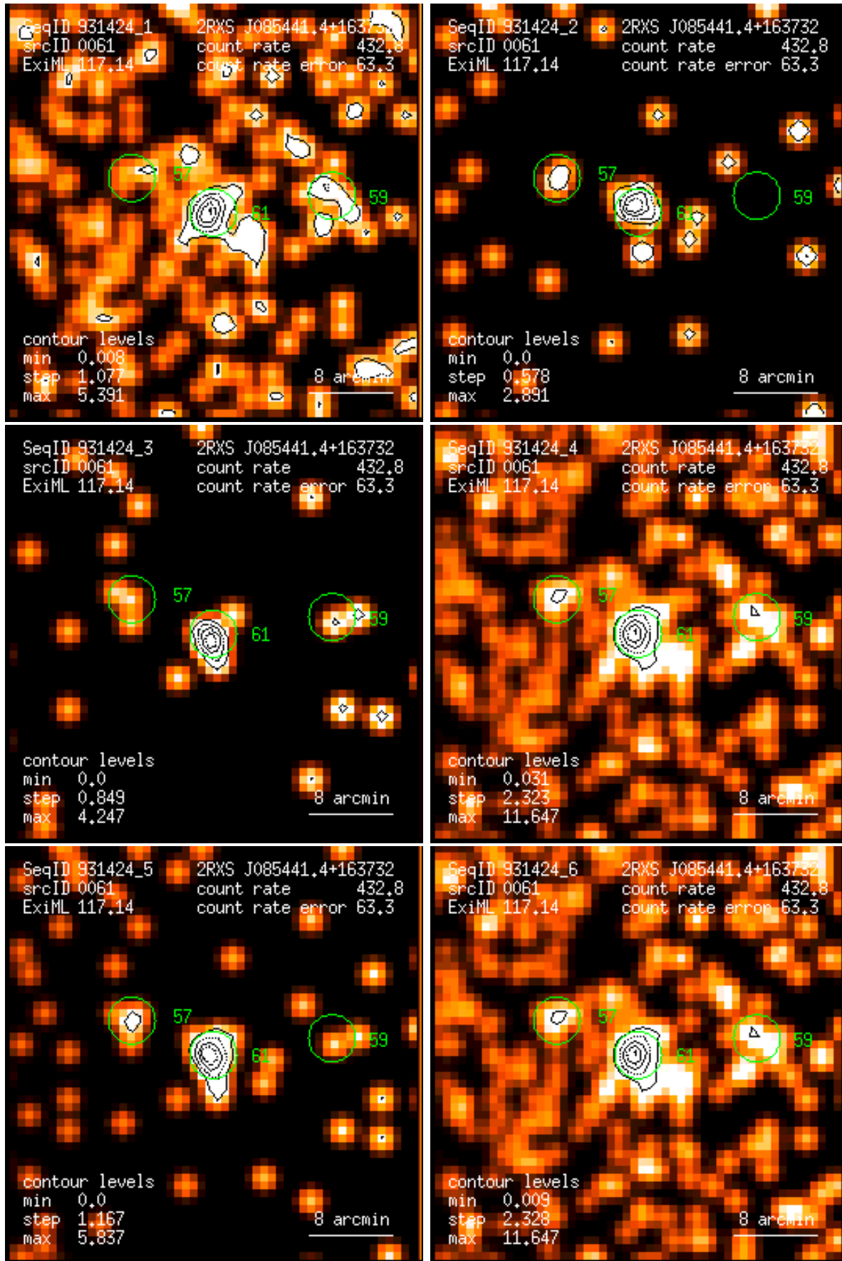
Figure 61: RASS 931424: detection 0061: band rate images, Gaussian filter: (1) PSPC channels 11 – 41, (2) 52 – 90, (3) 91 – 201, (4) 11 – 235, (5) 52 – 201, (6) 11 – 201. Broad band rates in counts/ks. Band rate contour levels in counts/ks/arcmin 2 .
